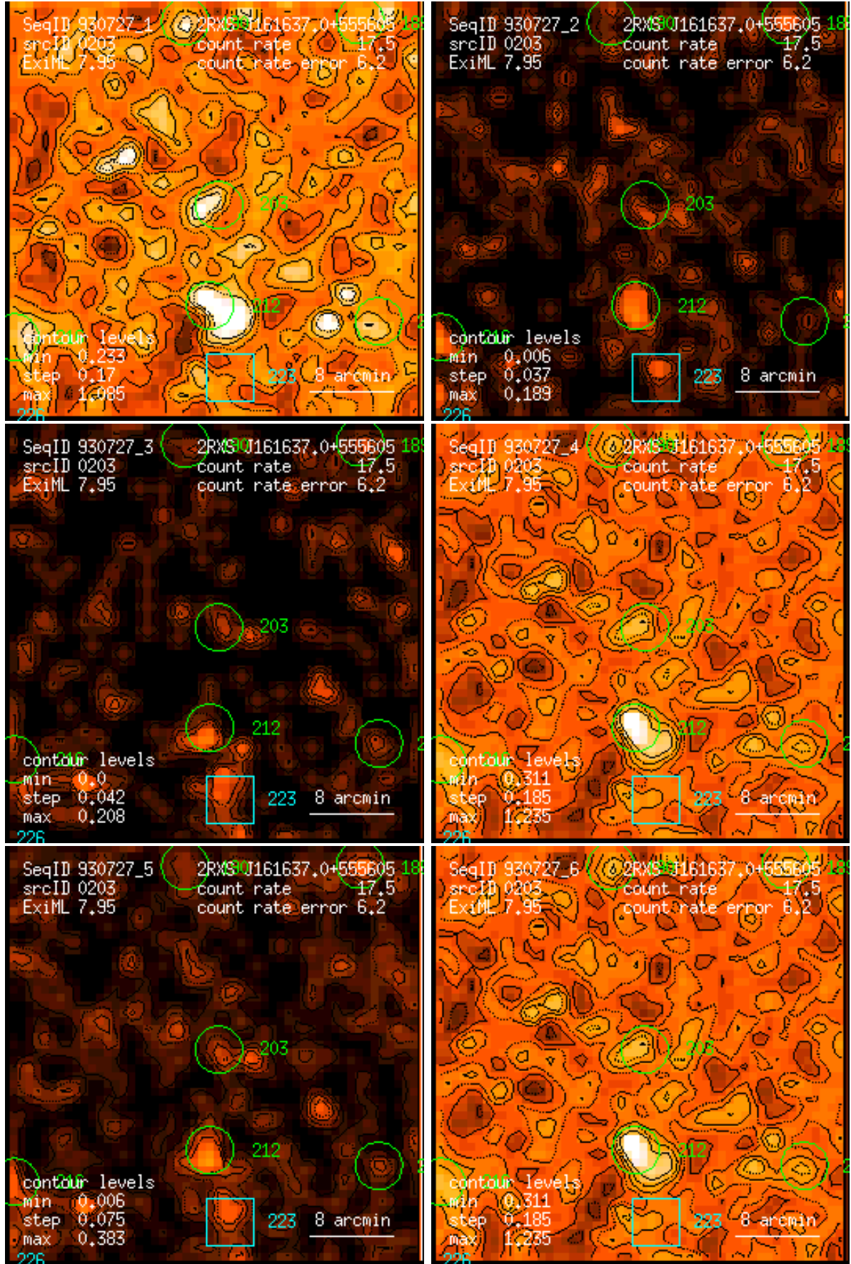
Figure 203: RASS 930727: detection 0203: band rate images, Gaussian filter: (1) PSPC channels 11 – 41, (2) 52 – 90, (3) 91 – 201, (4) 11 – 235, (5) 52 – 201, (6) 11 – 201. Broad band rates in counts/ks. Band rate contour levels in counts/ks/arcmin 2 .
