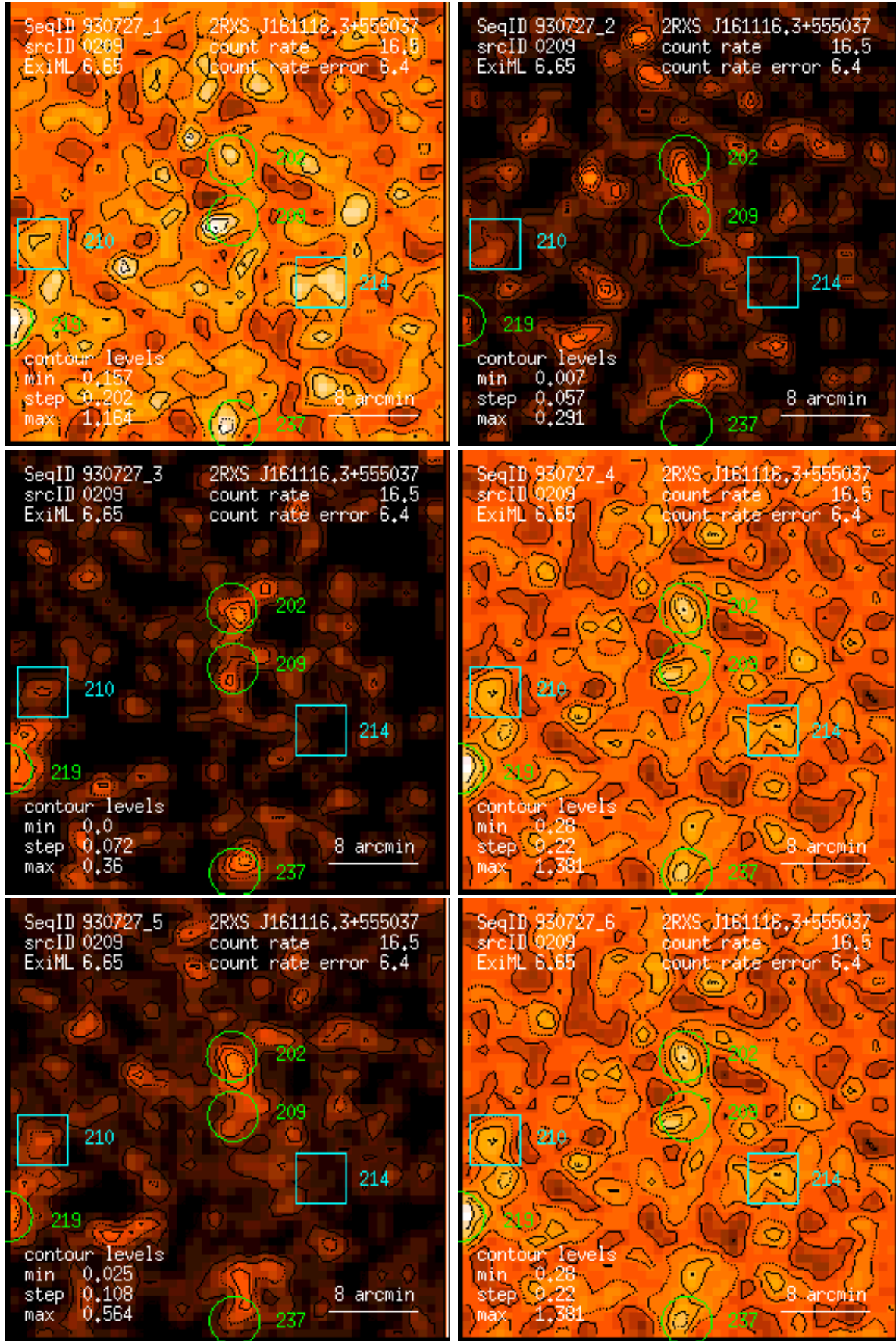
Figure 209: RASS 930727: detection 0209: band rate images, Gaussian filter: (1) PSPC channels 11 – 41, (2) 52 – 90, (3) 91 – 201, (4) 11 – 235, (5) 52 – 201, (6) 11 – 201. Broad band rates in counts/ks. Band rate contour levels in counts/ks/arcmin 2 .
