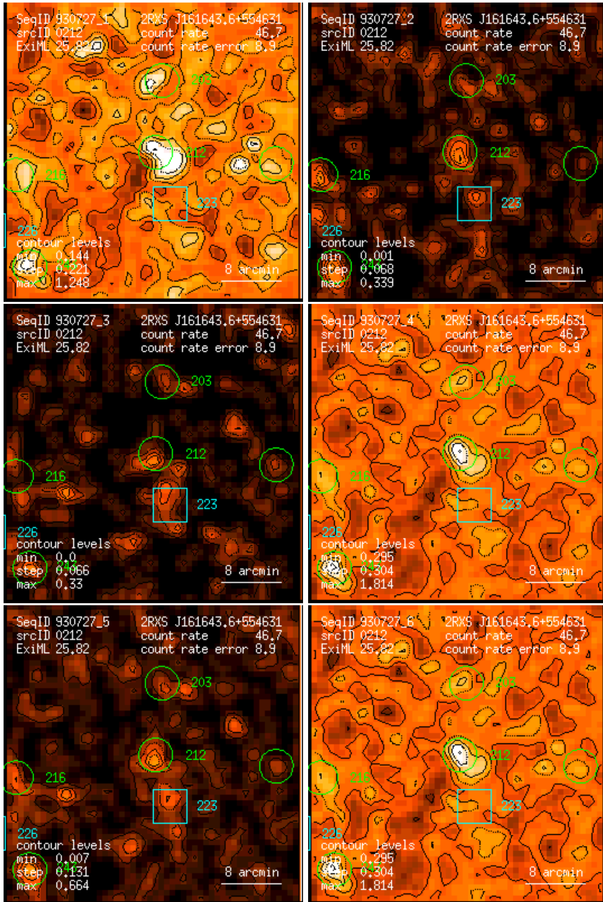
Figure 212: RASS 930727: detection 0212: band rate images, Gaussian filter: (1) PSPC channels 11 – 41, (2) 52 – 90, (3) 91 – 201, (4) 11 – 235, (5) 52 – 201, (6) 11 – 201. Broad band rates in counts/ks. Band rate contour levels in counts/ks/arcmin 2 .
