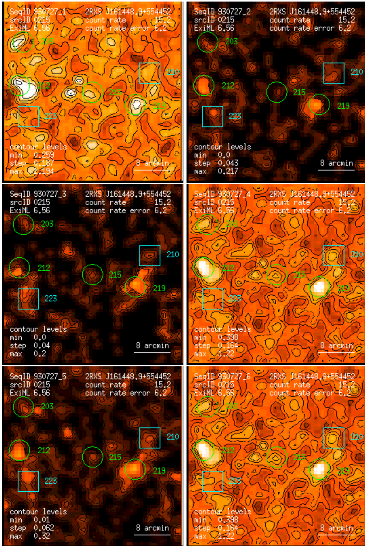
Figure 215: RASS 930727: detection 0215: band rate images, Gaussian filter: (1) PSPC channels 11 – 41, (2) 52 – 90, (3) 91 – 201, (4) 11 – 235, (5) 52 – 201, (6) 11 – 201. Broad band rates in counts/ks. Band rate contour levels in counts/ks/arcmin 2 .
