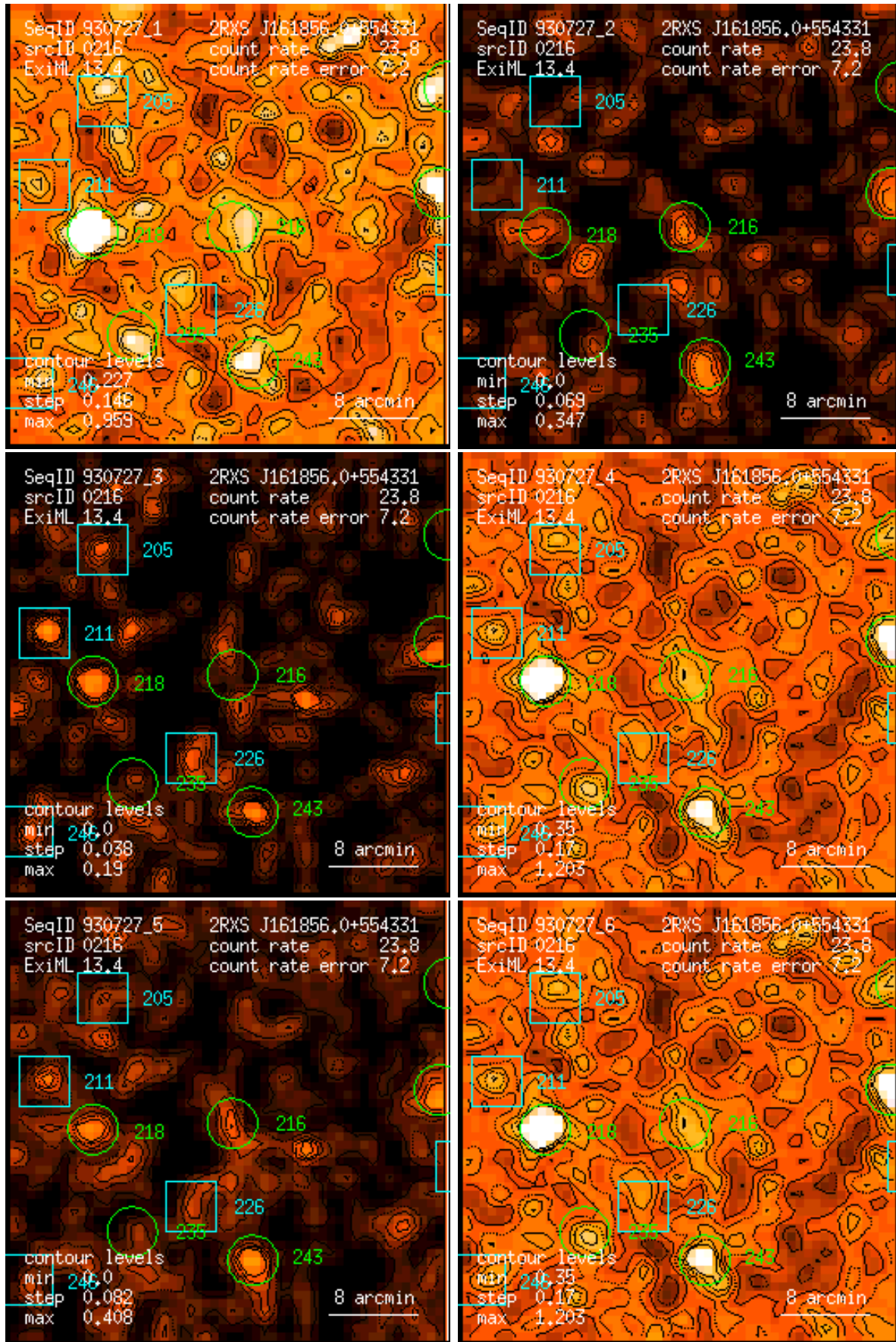
Figure 216: RASS 930727: detection 0216: band rate images, Gaussian filter: (1) PSPC channels 11 – 41, (2) 52 – 90, (3) 91 – 201, (4) 11 – 235, (5) 52 – 201, (6) 11 – 201. Broad band rates in counts/ks. Band rate contour levels in counts/ks/arcmin 2 .
