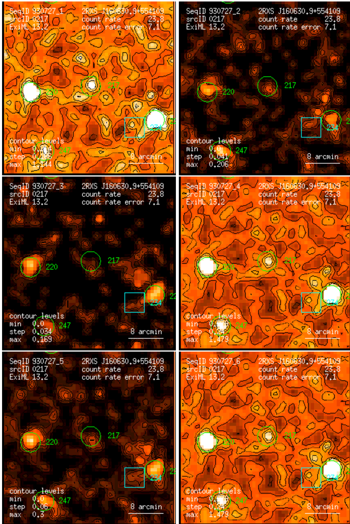
Figure 217: RASS 930727: detection 0217: band rate images, Gaussian filter: (1) PSPC channels 11 – 41, (2) 52 – 90, (3) 91 – 201, (4) 11 – 235, (5) 52 – 201, (6) 11 – 201. Broad band rates in counts/ks. Band rate contour levels in counts/ks/arcmin 2 .
