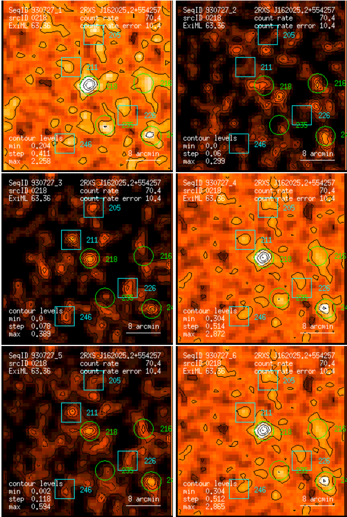
Figure 218: RASS 930727: detection 0218: band rate images, Gaussian filter: (1) PSPC channels 11 – 41, (2) 52 – 90, (3) 91 – 201, (4) 11 – 235, (5) 52 – 201, (6) 11 – 201. Broad band rates in counts/ks. Band rate contour levels in counts/ks/arcmin 2 .
