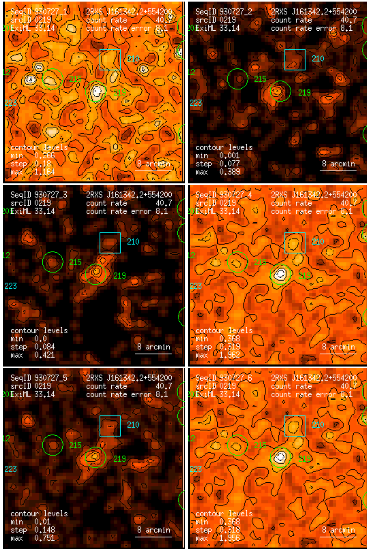
Figure 219: RASS 930727: detection 0219: band rate images, Gaussian filter: (1) PSPC channels 11 – 41, (2) 52 – 90, (3) 91 – 201, (4) 11 – 235, (5) 52 – 201, (6) 11 – 201. Broad band rates in counts/ks. Band rate contour levels in counts/ks/arcmin 2 .
