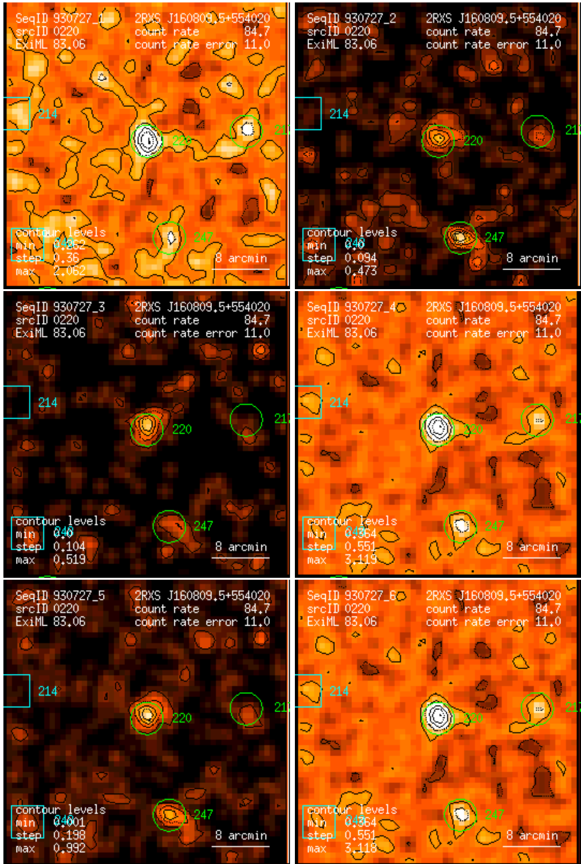
Figure 220: RASS 930727: detection 0220: band rate images, Gaussian filter: (1) PSPC channels 11 – 41, (2) 52 – 90, (3) 91 – 201, (4) 11 – 235, (5) 52 – 201, (6) 11 – 201. Broad band rates in counts/ks. Band rate contour levels in counts/ks/arcmin 2 .
