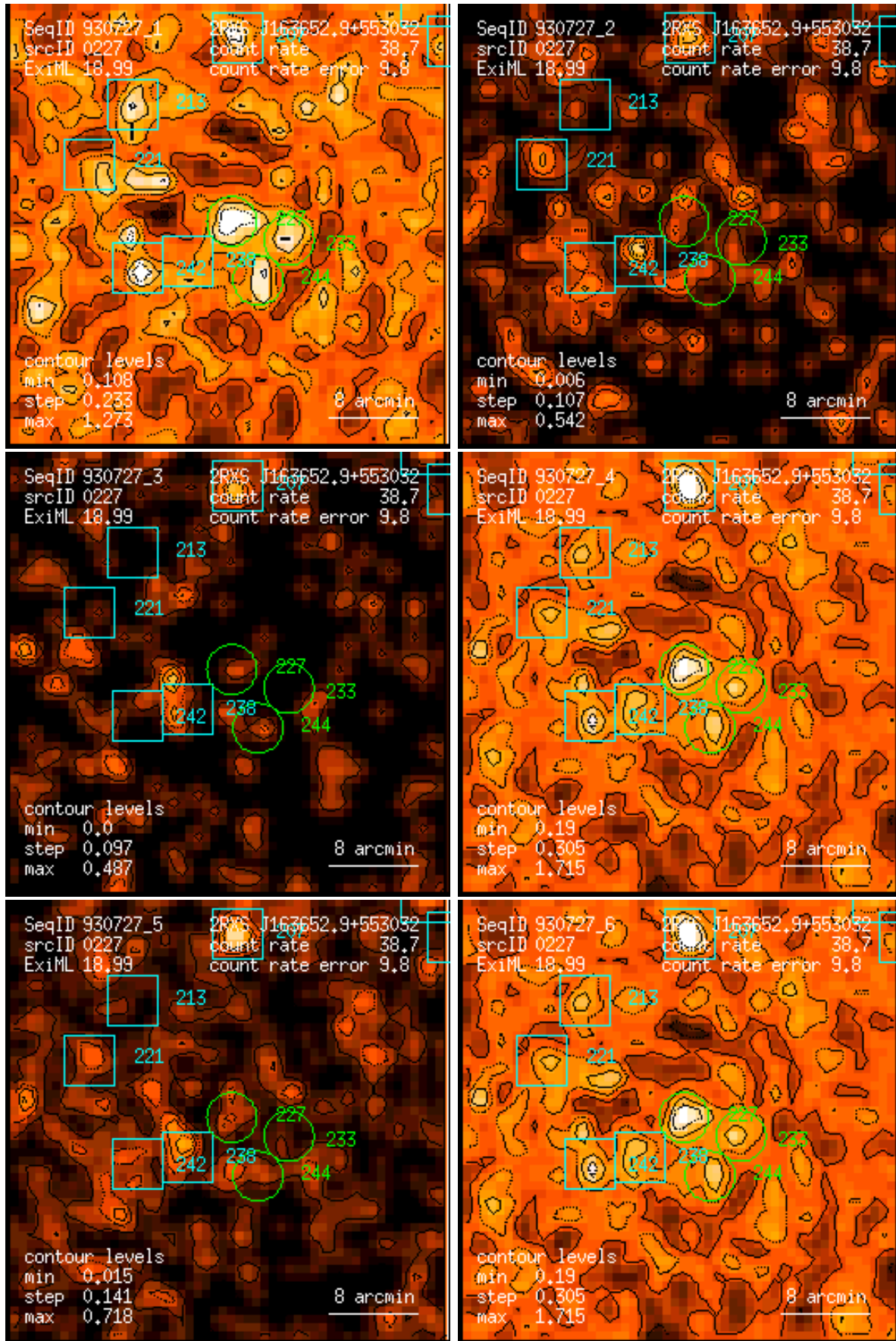
Figure 227: RASS 930727: detection 0227: band rate images, Gaussian filter: (1) PSPC channels 11 – 41, (2) 52 – 90, (3) 91 – 201, (4) 11 – 235, (5) 52 – 201, (6) 11 – 201. Broad band rates in counts/ks. Band rate contour levels in counts/ks/arcmin 2 .
