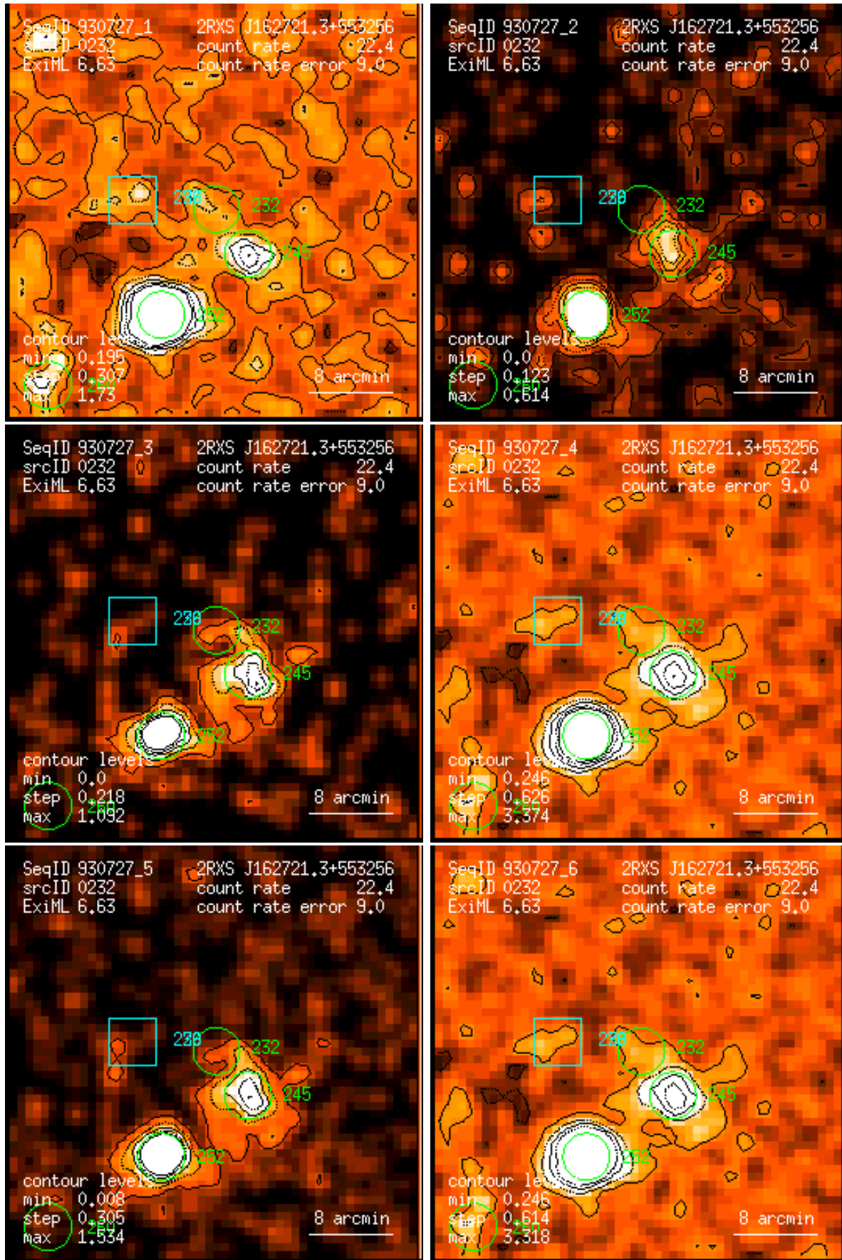
Figure 232: RASS 930727: detection 0232: band rate images, Gaussian filter: (1) PSPC channels 11 – 41, (2) 52 – 90, (3) 91 – 201, (4) 11 – 235, (5) 52 – 201, (6) 11 – 201. Broad band rates in counts/ks. Band rate contour levels in counts/ks/arcmin 2 .
