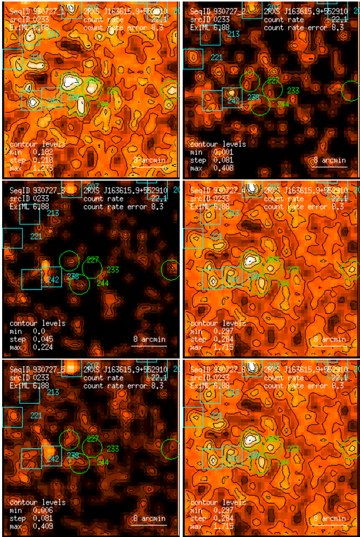
Figure 233: RASS 930727: detection 0233: band rate images, Gaussian filter: (1) PSPC channels 11 – 41, (2) 52 – 90, (3) 91 – 201, (4) 11 – 235, (5) 52 – 201, (6) 11 – 201. Broad band rates in counts/ks. Band rate contour levels in counts/ks/arcmin 2 .
