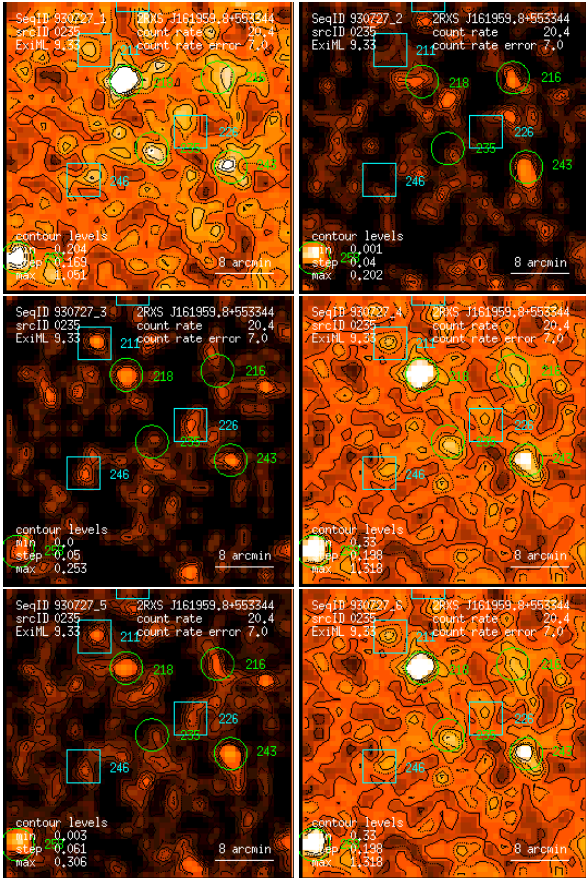
Figure 235: RASS 930727: detection 0235: band rate images, Gaussian filter: (1) PSPC channels 11 – 41, (2) 52 – 90, (3) 91 – 201, (4) 11 – 235, (5) 52 – 201, (6) 11 – 201. Broad band rates in counts/ks. Band rate contour levels in counts/ks/arcmin 2 .
