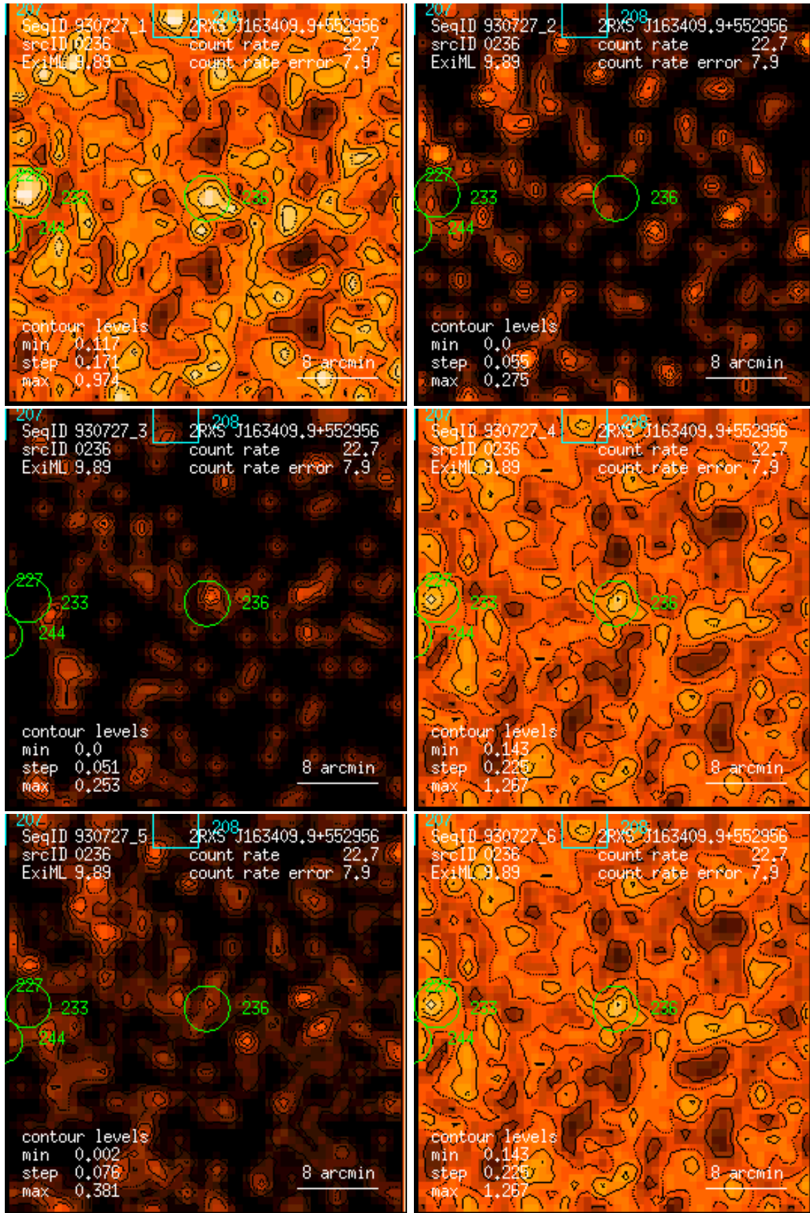
Figure 236: RASS 930727: detection 0236: band rate images, Gaussian filter: (1) PSPC channels 11 – 41, (2) 52 – 90, (3) 91 – 201, (4) 11 – 235, (5) 52 – 201, (6) 11 – 201. Broad band rates in counts/ks. Band rate contour levels in counts/ks/arcmin 2 .
