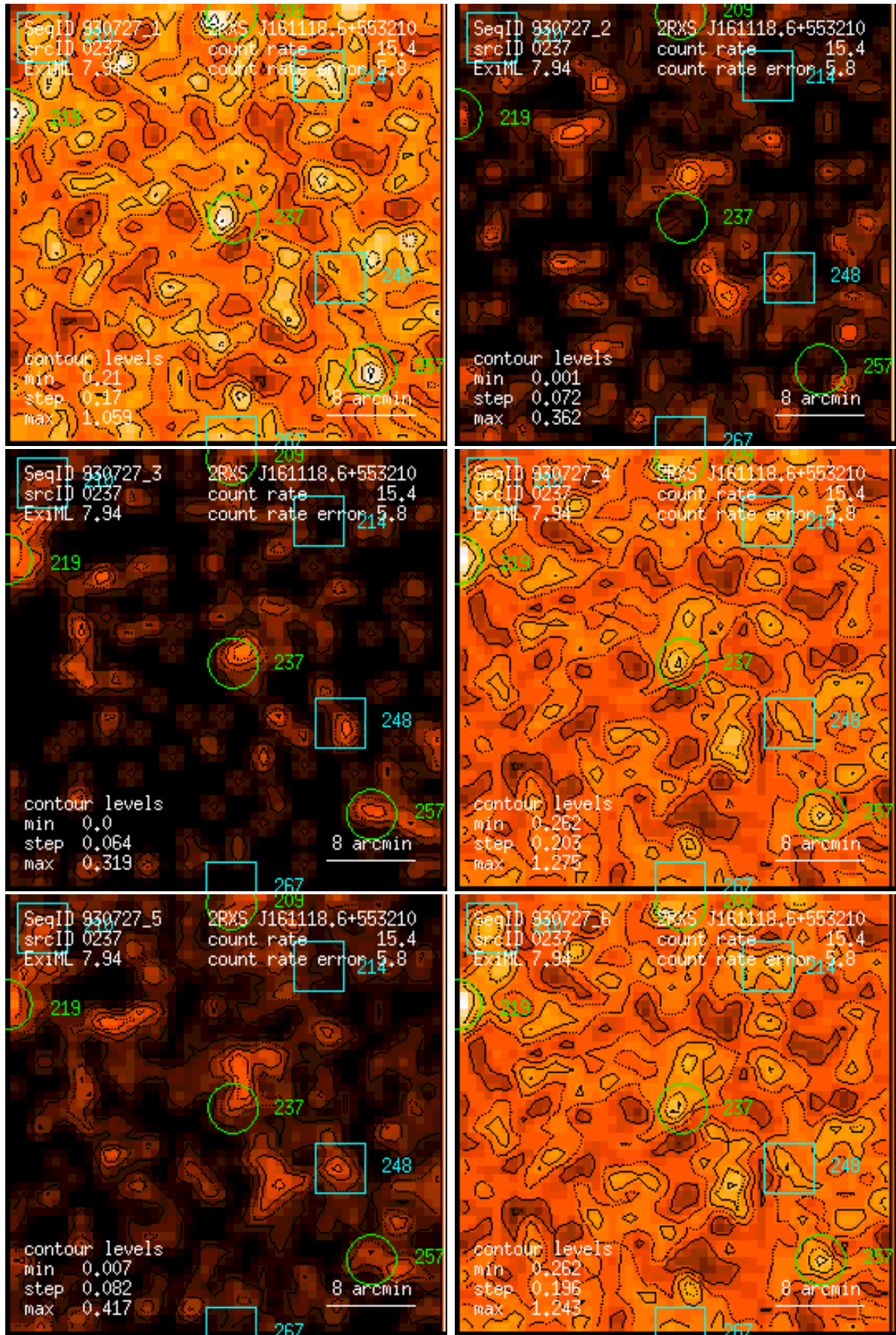
Figure 237: RASS 930727: detection 0237: band rate images, Gaussian filter: (1) PSPC channels 11 – 41, (2) 52 – 90, (3) 91 – 201, (4) 11 – 235, (5) 52 – 201, (6) 11 – 201. Broad band rates in counts/ks. Band rate contour levels in counts/ks/arcmin 2 .
