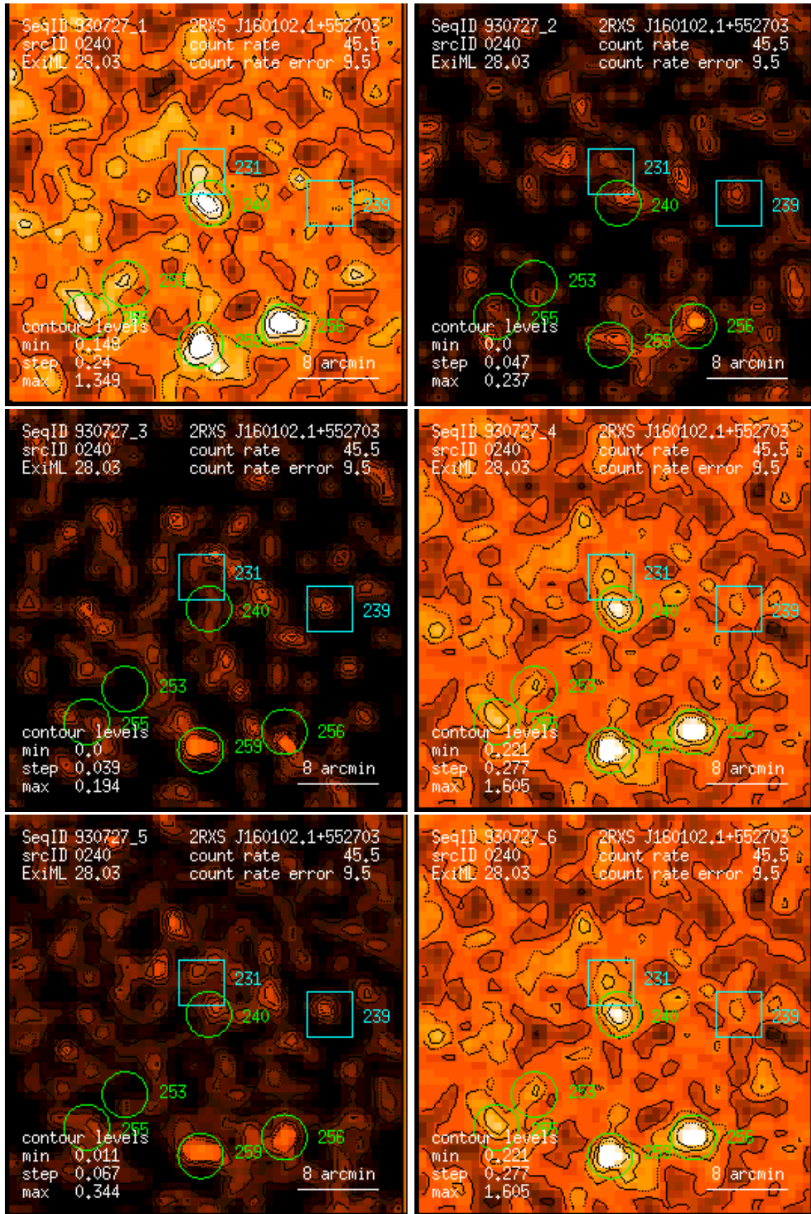
Figure 240: RASS 930727: detection 0240: band rate images, Gaussian filter: (1) PSPC channels 11 – 41, (2) 52 – 90, (3) 91 – 201, (4) 11 – 235, (5) 52 – 201, (6) 11 – 201. Broad band rates in counts/ks. Band rate contour levels in counts/ks/arcmin 2 .
