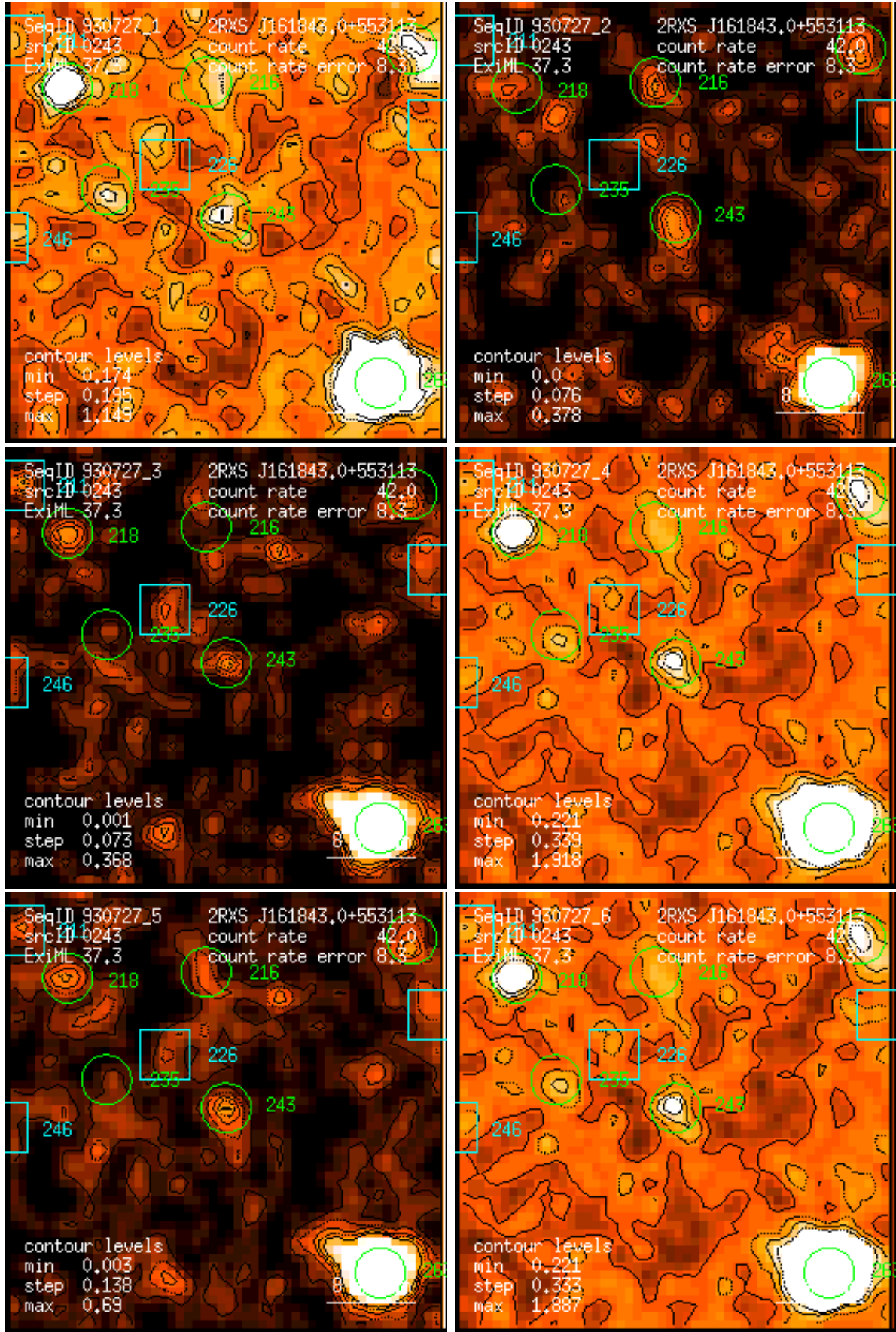
Figure 243: RASS 930727: detection 0243: band rate images, Gaussian filter: (1) PSPC channels 11 – 41, (2) 52 – 90, (3) 91 – 201, (4) 11 – 235, (5) 52 – 201, (6) 11 – 201. Broad band rates in counts/ks. Band rate contour levels in counts/ks/arcmin 2 .
