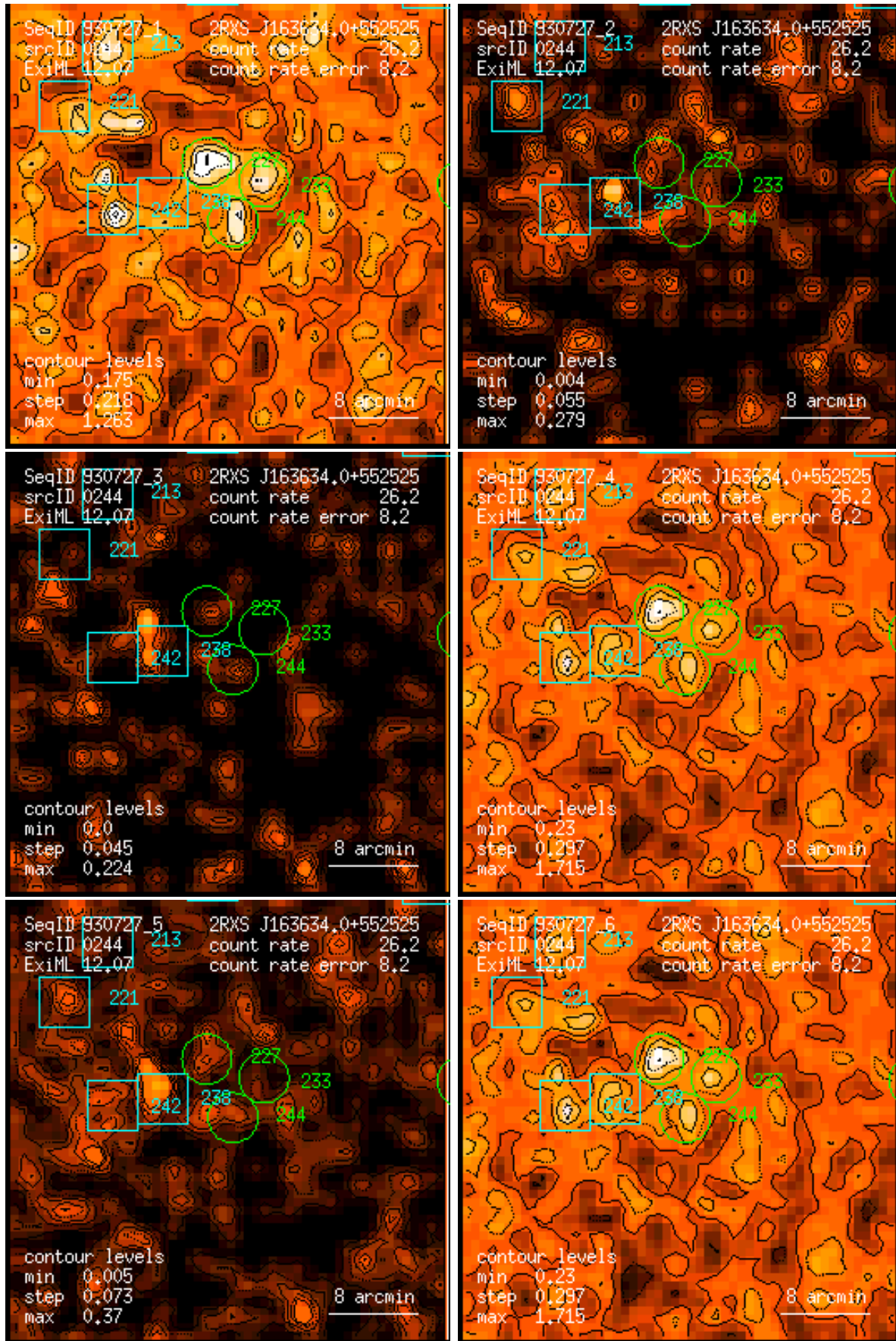
Figure 244: RASS 930727: detection 0244: band rate images, Gaussian filter: (1) PSPC channels 11 – 41, (2) 52 – 90, (3) 91 – 201, (4) 11 – 235, (5) 52 – 201, (6) 11 – 201. Broad band rates in counts/ks. Band rate contour levels in counts/ks/arcmin 2 .
