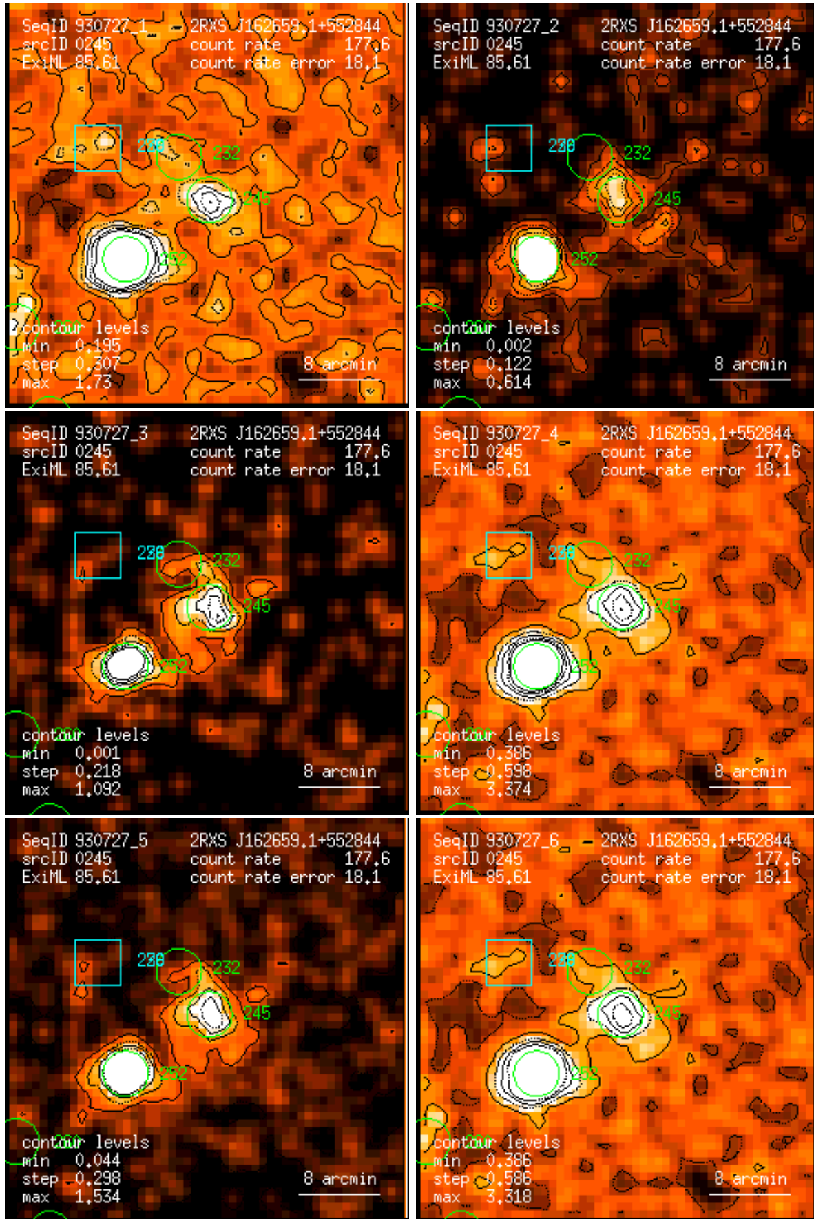
Figure 245: RASS 930727: detection 0245: band rate images, Gaussian filter: (1) PSPC channels 11 – 41, (2) 52 – 90, (3) 91 – 201, (4) 11 – 235, (5) 52 – 201, (6) 11 – 201. Broad band rates in counts/ks. Band rate contour levels in counts/ks/arcmin 2 .
