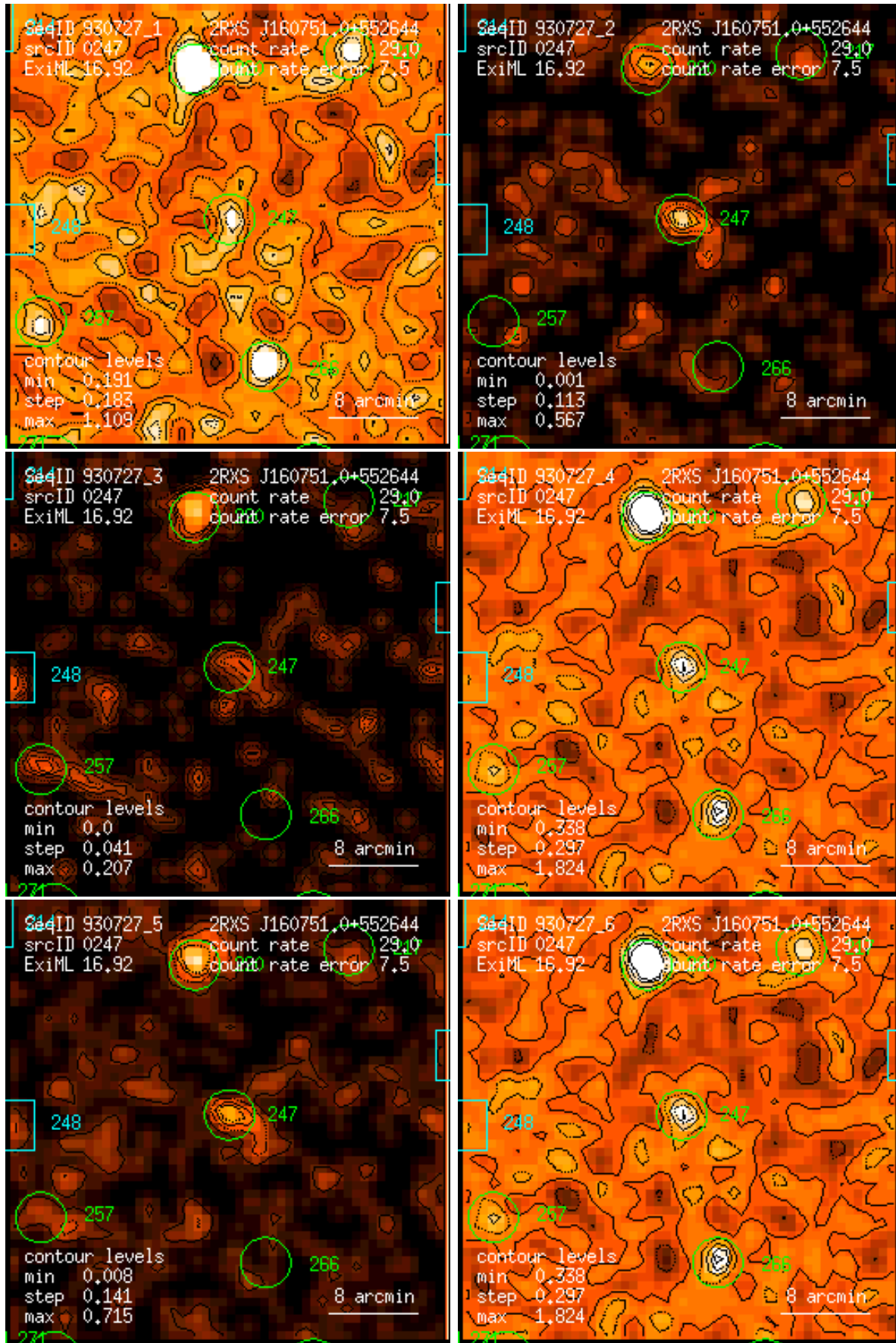
Figure 247: RASS 930727: detection 0247: band rate images, Gaussian filter: (1) PSPC channels 11 – 41, (2) 52 – 90, (3) 91 – 201, (4) 11 – 235, (5) 52 – 201, (6) 11 – 201. Broad band rates in counts/ks. Band rate contour levels in counts/ks/arcmin 2 .
