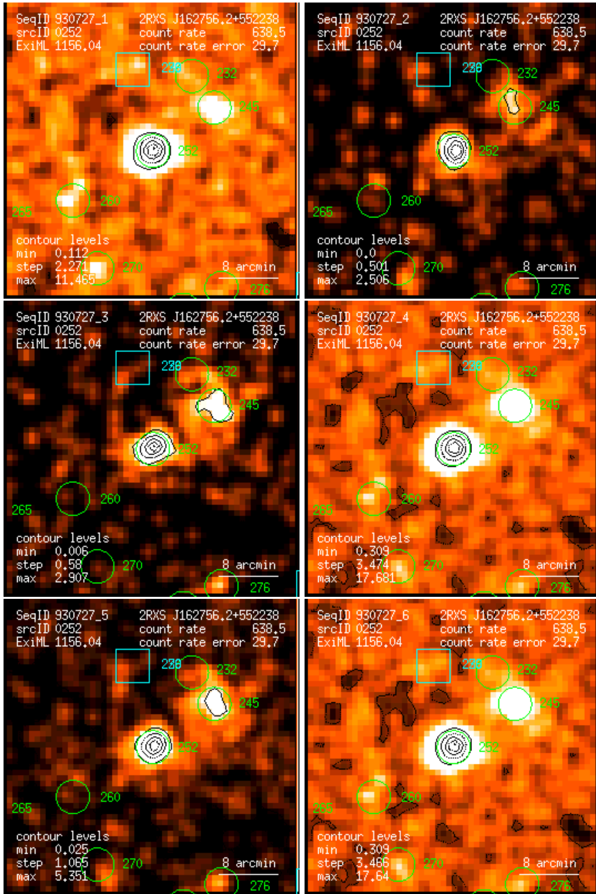
Figure 252: RASS 930727: detection 0252: band rate images, Gaussian filter: (1) PSPC channels 11 – 41, (2) 52 – 90, (3) 91 – 201, (4) 11 – 235, (5) 52 – 201, (6) 11 – 201. Broad band rates in counts/ks. Band rate contour levels in counts/ks/arcmin 2 .
