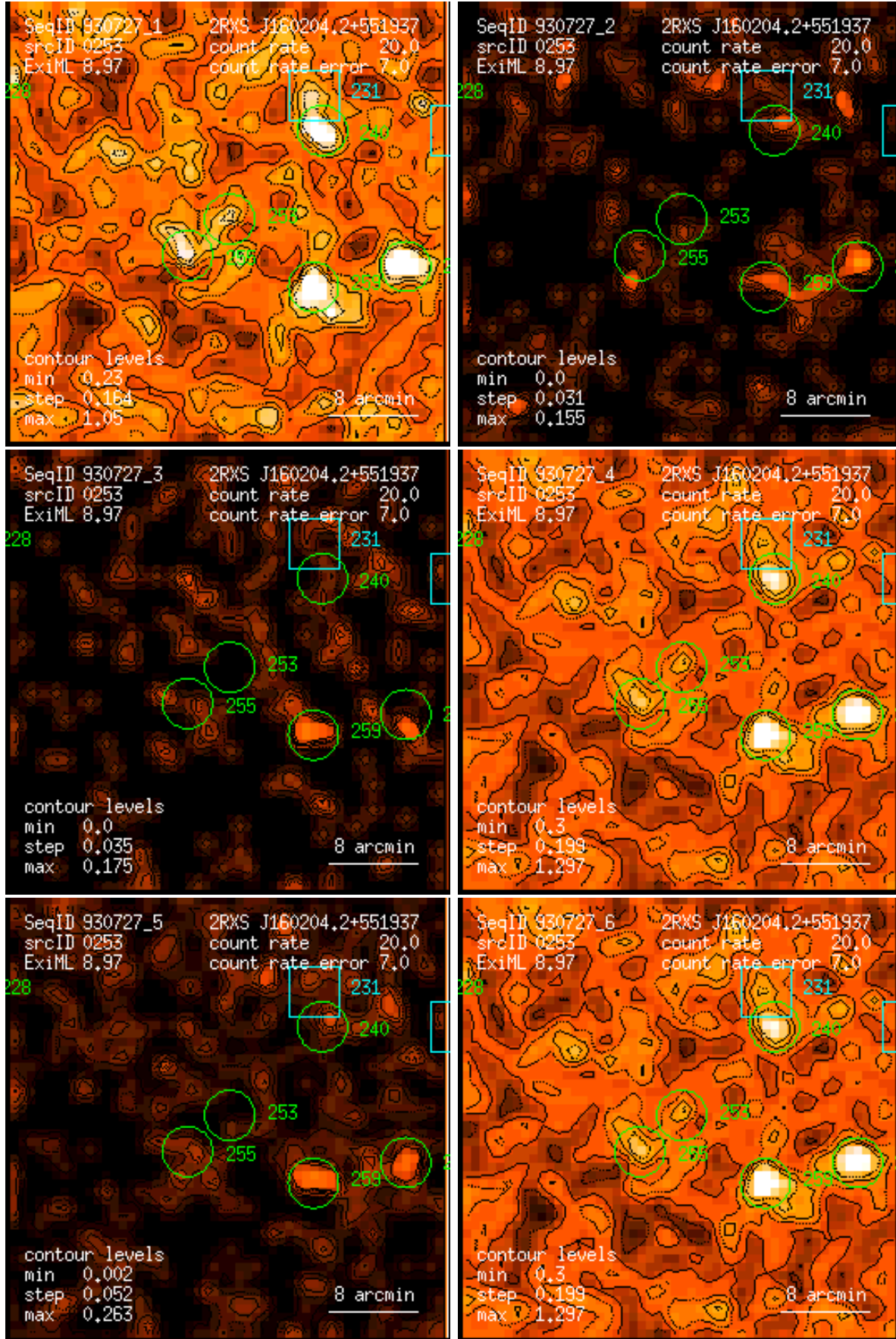
Figure 253: RASS 930727: detection 0253: band rate images, Gaussian filter: (1) PSPC channels 11 – 41, (2) 52 – 90, (3) 91 – 201, (4) 11 – 235, (5) 52 – 201, (6) 11 – 201. Broad band rates in counts/ks. Band rate contour levels in counts/ks/arcmin 2 .
