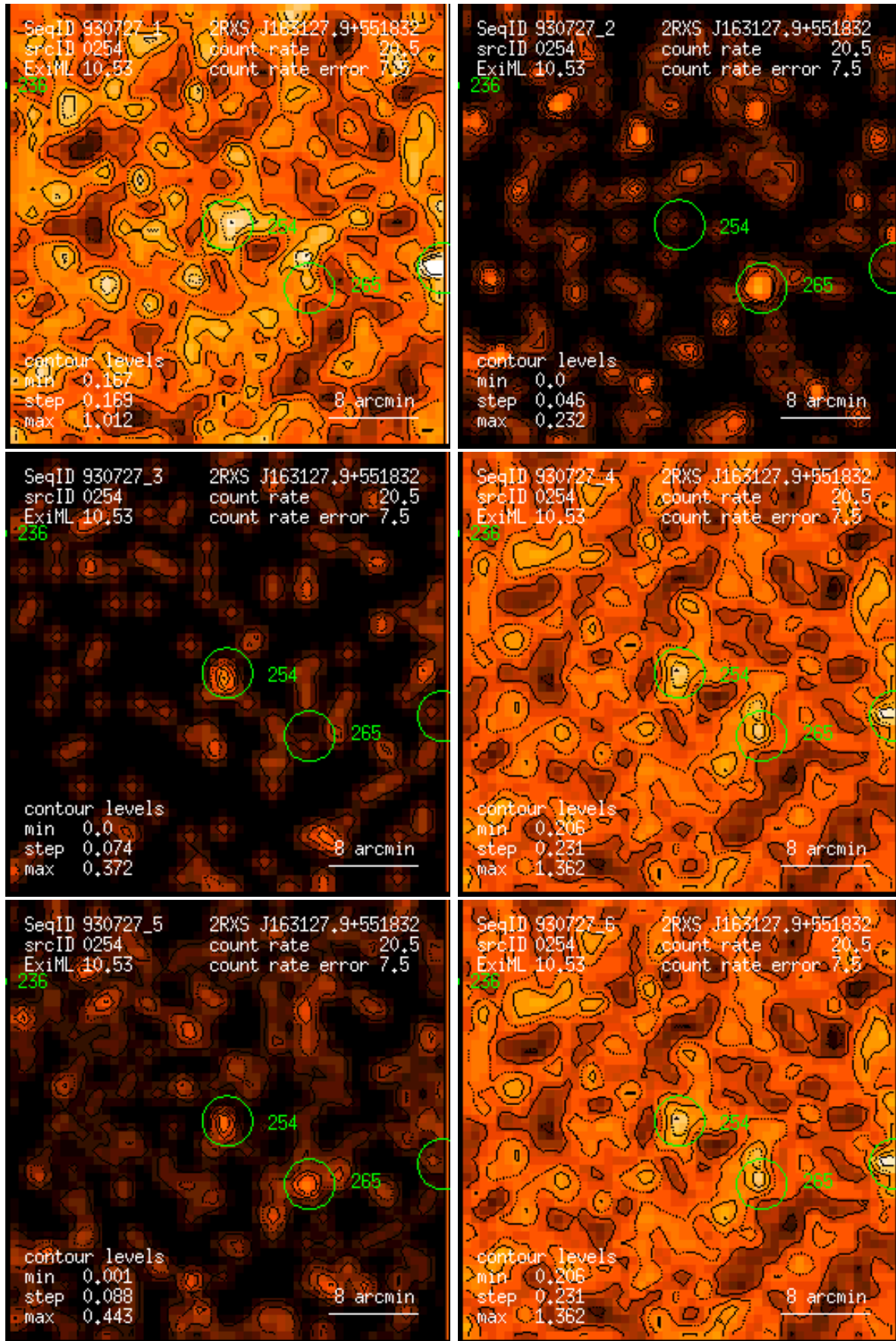
Figure 254: RASS 930727: detection 0254: band rate images, Gaussian filter: (1) PSPC channels 11 – 41, (2) 52 – 90, (3) 91 – 201, (4) 11 – 235, (5) 52 – 201, (6) 11 – 201. Broad band rates in counts/ks. Band rate contour levels in counts/ks/arcmin 2 .
