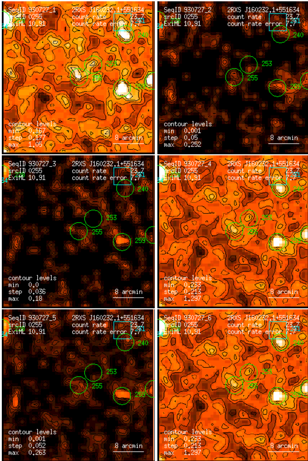
Figure 255: RASS 930727: detection 0255: band rate images, Gaussian filter: (1) PSPC channels 11 – 41, (2) 52 – 90, (3) 91 – 201, (4) 11 – 235, (5) 52 – 201, (6) 11 – 201. Broad band rates in counts/ks. Band rate contour levels in counts/ks/arcmin 2 .
