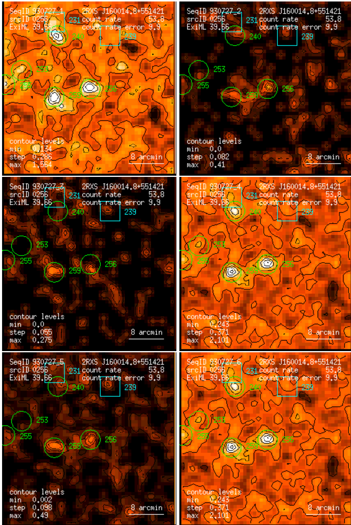
Figure 256: RASS 930727: detection 0256: band rate images, Gaussian filter: (1) PSPC channels 11 – 41, (2) 52 – 90, (3) 91 – 201, (4) 11 – 235, (5) 52 – 201, (6) 11 – 201. Broad band rates in counts/ks. Band rate contour levels in counts/ks/arcmin 2 .
