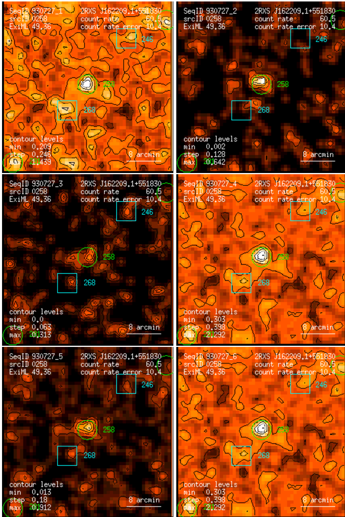
Figure 258: RASS 930727: detection 0258: band rate images, Gaussian filter: (1) PSPC channels 11 – 41, (2) 52 – 90, (3) 91 – 201, (4) 11 – 235, (5) 52 – 201, (6) 11 – 201. Broad band rates in counts/ks. Band rate contour levels in counts/ks/arcmin 2 .
