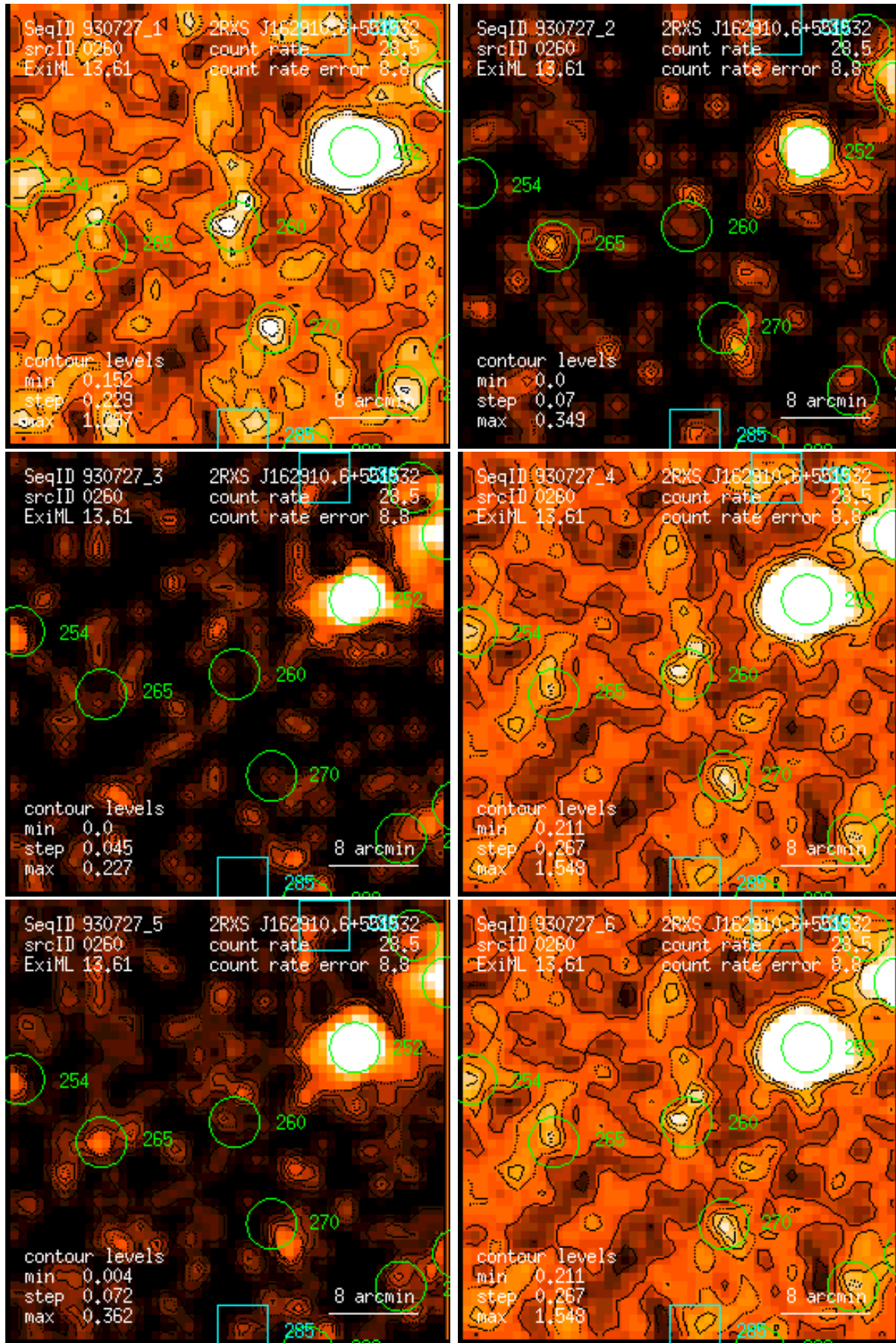
Figure 260: RASS 930727: detection 0260: band rate images, Gaussian filter: (1) PSPC channels 11 – 41, (2) 52 – 90, (3) 91 – 201, (4) 11 – 235, (5) 52 – 201, (6) 11 – 201. Broad band rates in counts/ks. Band rate contour levels in counts/ks/arcmin 2 .
