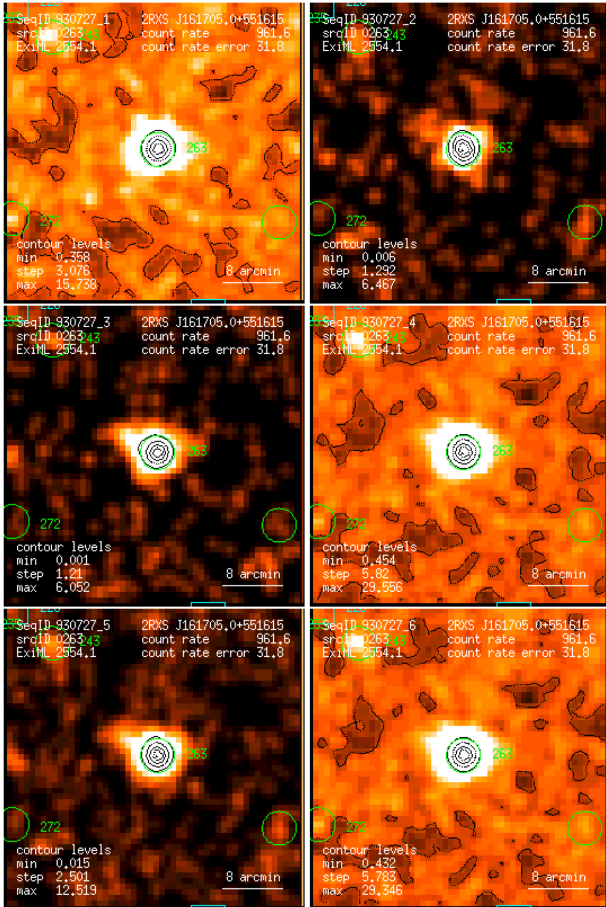
Figure 263: RASS 930727: detection 0263: band rate images, Gaussian filter: (1) PSPC channels 11 – 41, (2) 52 – 90, (3) 91 – 201, (4) 11 – 235, (5) 52 – 201, (6) 11 – 201. Broad band rates in counts/ks. Band rate contour levels in counts/ks/arcmin 2 .
