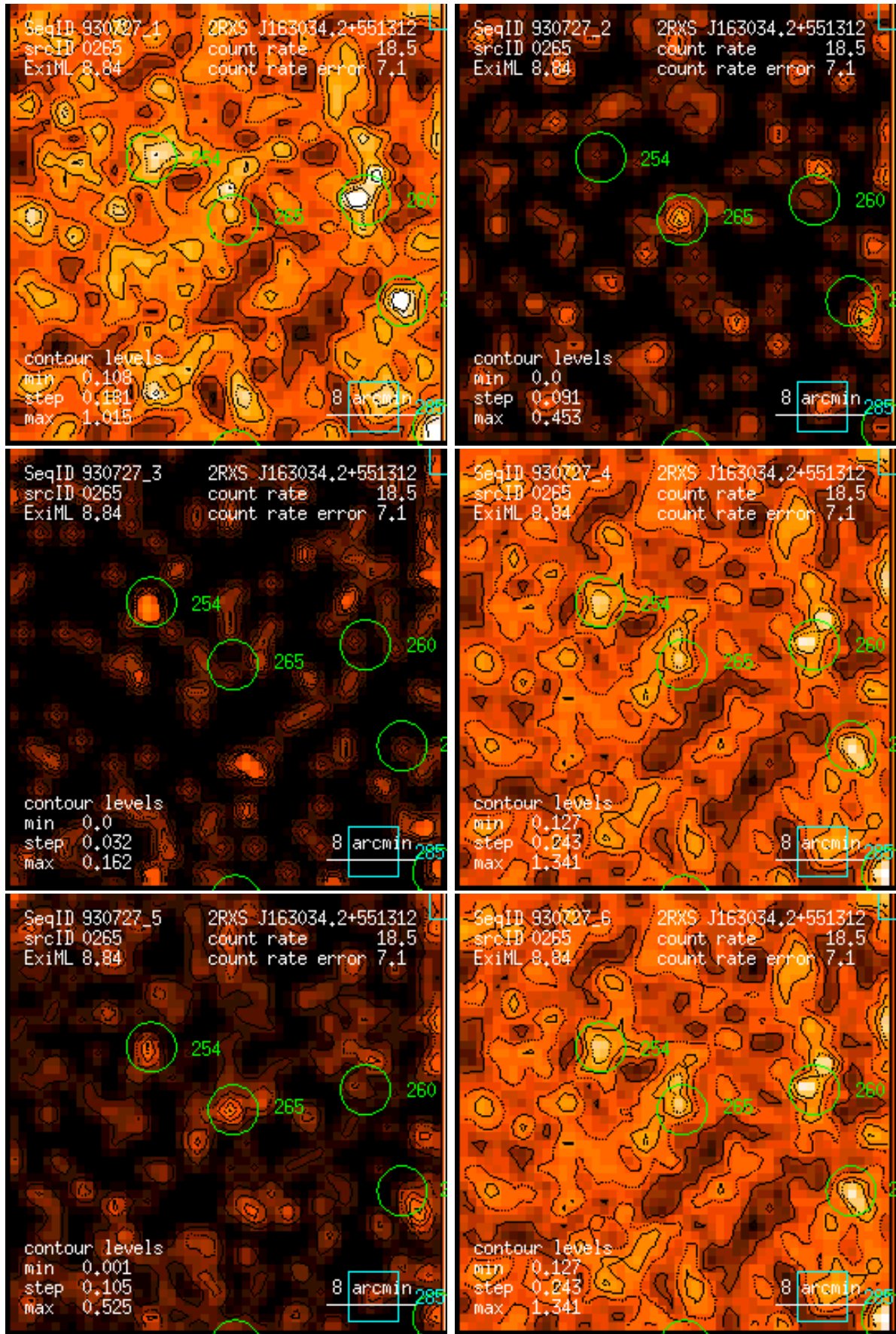
Figure 265: RASS 930727: detection 0265: band rate images, Gaussian filter: (1) PSPC channels 11 – 41, (2) 52 – 90, (3) 91 – 201, (4) 11 – 235, (5) 52 – 201, (6) 11 – 201. Broad band rates in counts/ks. Band rate contour levels in counts/ks/arcmin 2 .
