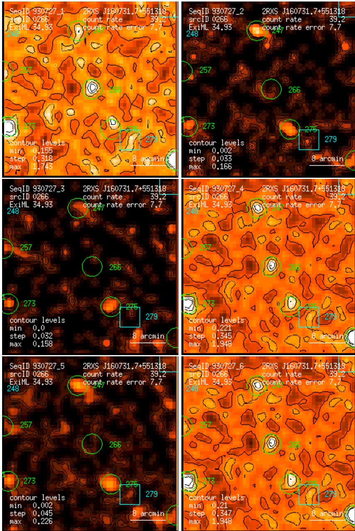
Figure 266: RASS 930727: detection 0266: band rate images, Gaussian filter: (1) PSPC channels 11 – 41, (2) 52 – 90, (3) 91 – 201, (4) 11 – 235, (5) 52 – 201, (6) 11 – 201. Broad band rates in counts/ks. Band rate contour levels in counts/ks/arcmin 2 .
