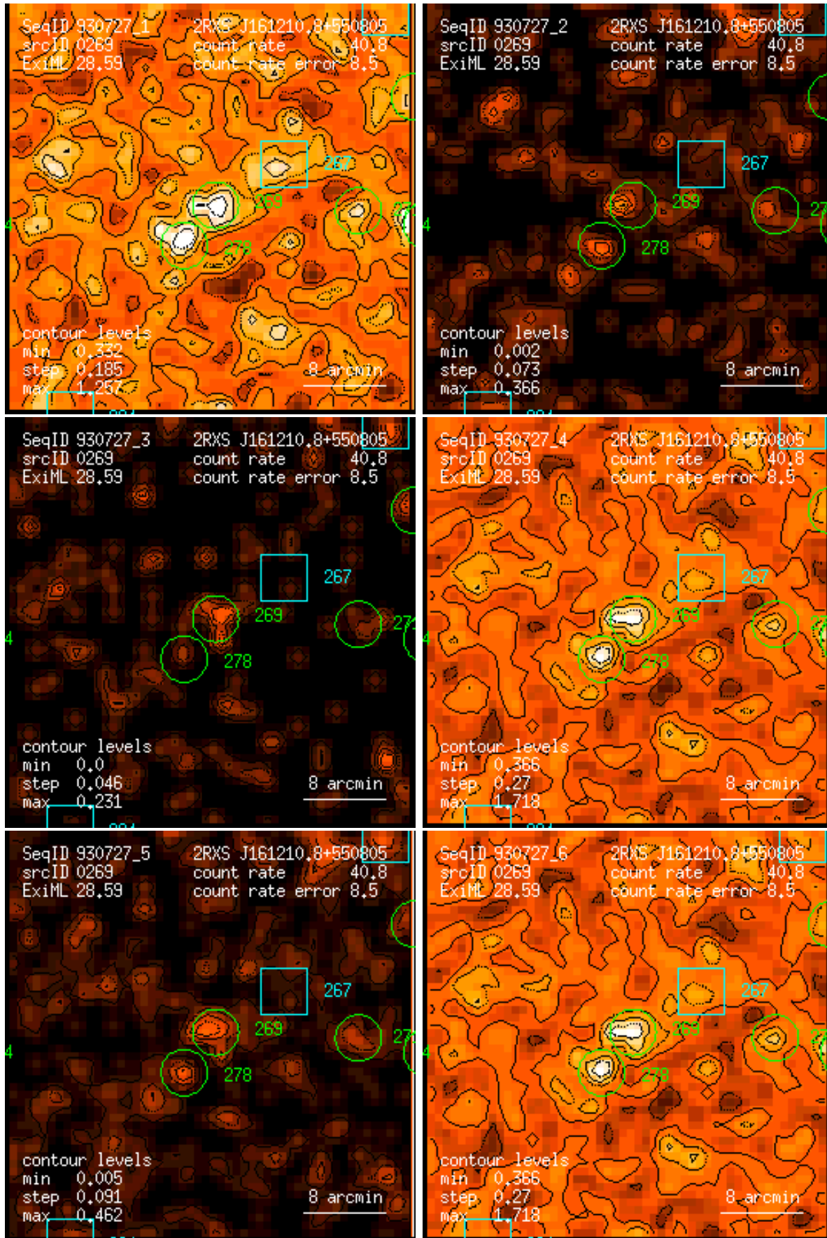
Figure 269: RASS 930727: detection 0269: band rate images, Gaussian filter: (1) PSPC channels 11 – 41, (2) 52 – 90, (3) 91 – 201, (4) 11 – 235, (5) 52 – 201, (6) 11 – 201. Broad band rates in counts/ks. Band rate contour levels in counts/ks/arcmin 2 .
