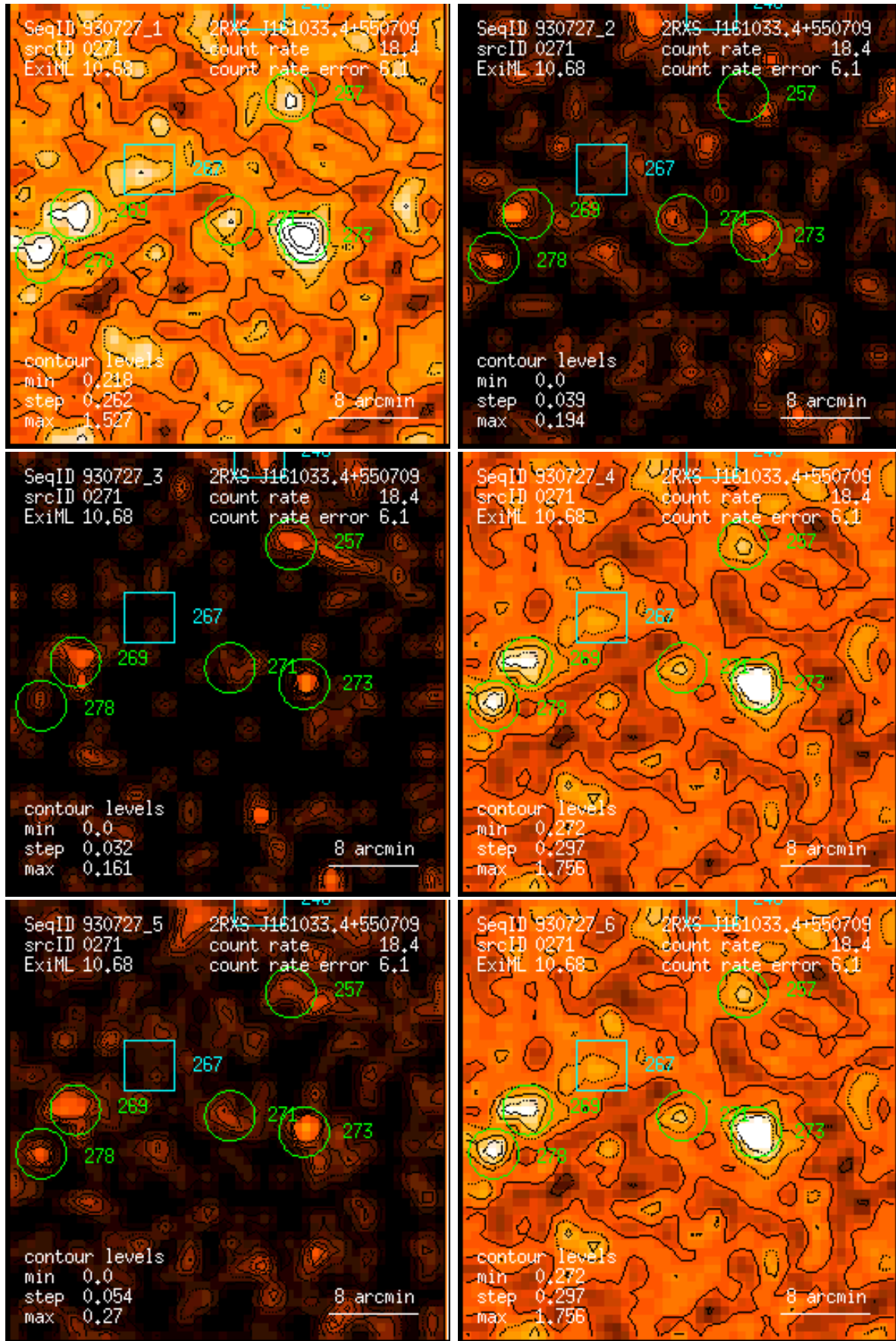
Figure 271: RASS 930727: detection 0271: band rate images, Gaussian filter: (1) PSPC channels 11 – 41, (2) 52 – 90, (3) 91 – 201, (4) 11 – 235, (5) 52 – 201, (6) 11 – 201. Broad band rates in counts/ks. Band rate contour levels in counts/ks/arcmin 2 .
