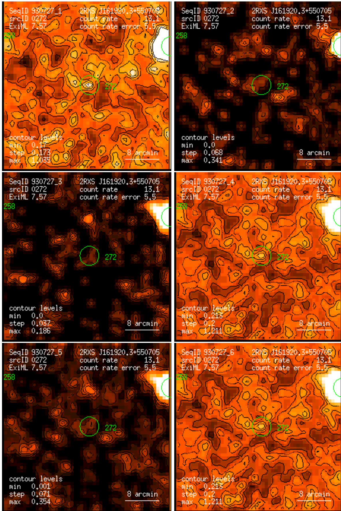
Figure 272: RASS 930727: detection 0272: band rate images, Gaussian filter: (1) PSPC channels 11 – 41, (2) 52 – 90, (3) 91 – 201, (4) 11 – 235, (5) 52 – 201, (6) 11 – 201. Broad band rates in counts/ks. Band rate contour levels in counts/ks/arcmin 2 .
