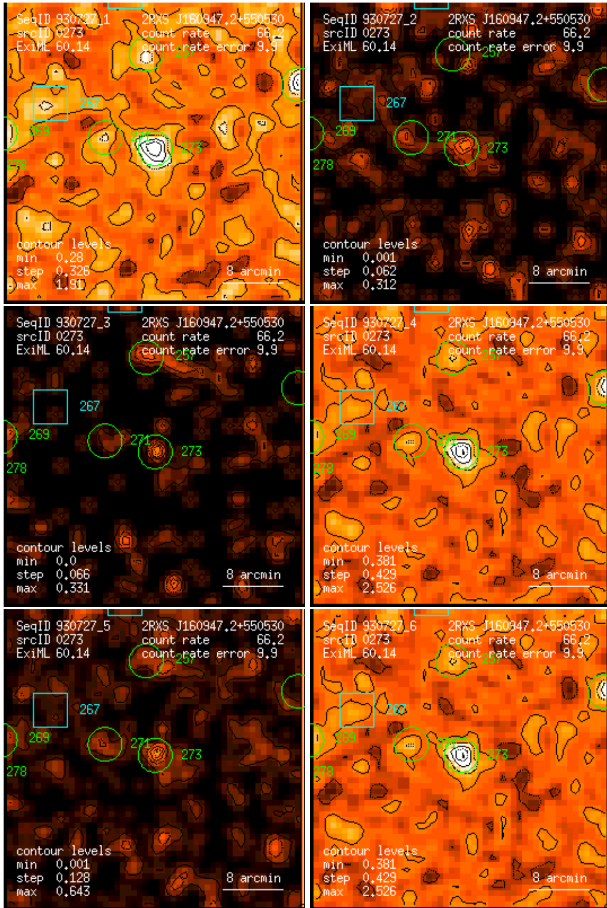
Figure 273: RASS 930727: detection 0273: band rate images, Gaussian filter: (1) PSPC channels 11 – 41, (2) 52 – 90, (3) 91 – 201, (4) 11 – 235, (5) 52 – 201, (6) 11 – 201. Broad band rates in counts/ks. Band rate contour levels in counts/ks/arcmin 2 .
