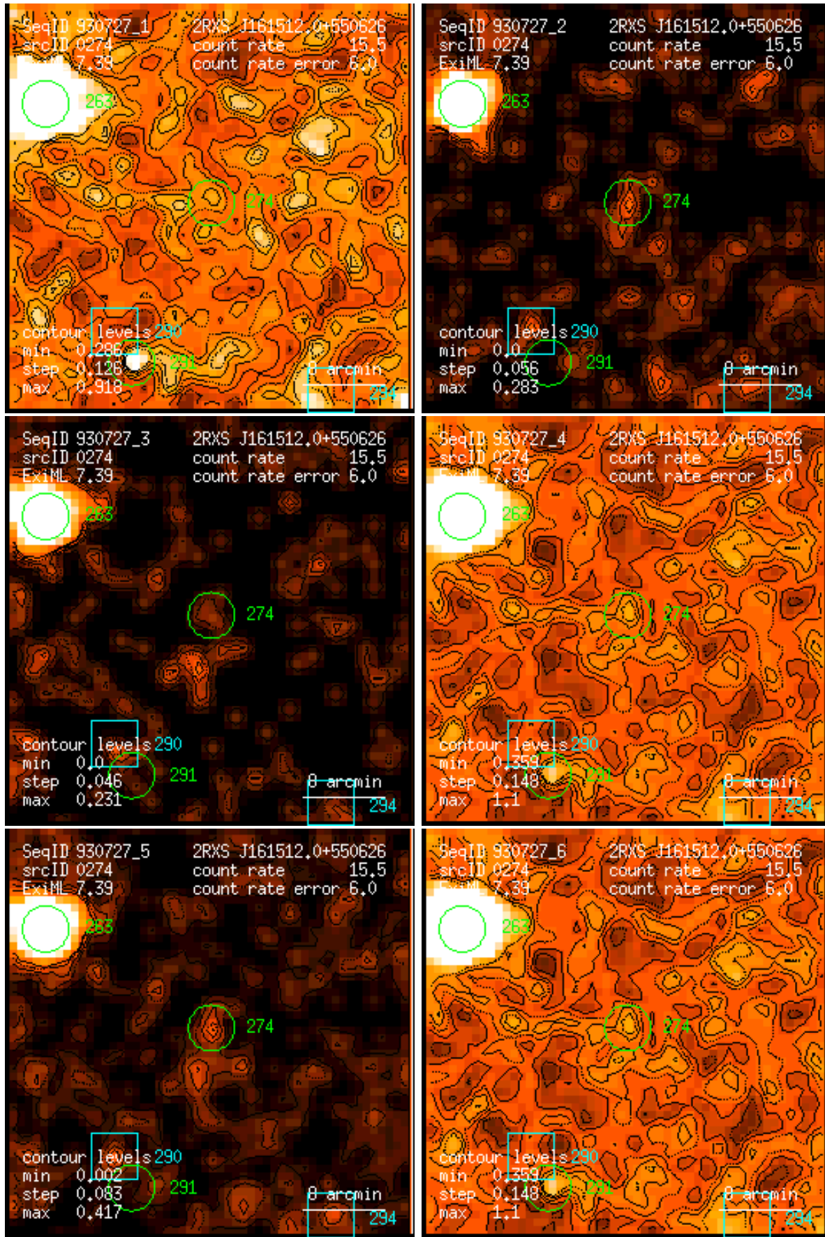
Figure 274: RASS 930727: detection 0274: band rate images, Gaussian filter: (1) PSPC channels 11 – 41, (2) 52 – 90, (3) 91 – 201, (4) 11 – 235, (5) 52 – 201, (6) 11 – 201. Broad band rates in counts/ks. Band rate contour levels in counts/ks/arcmin 2 .
