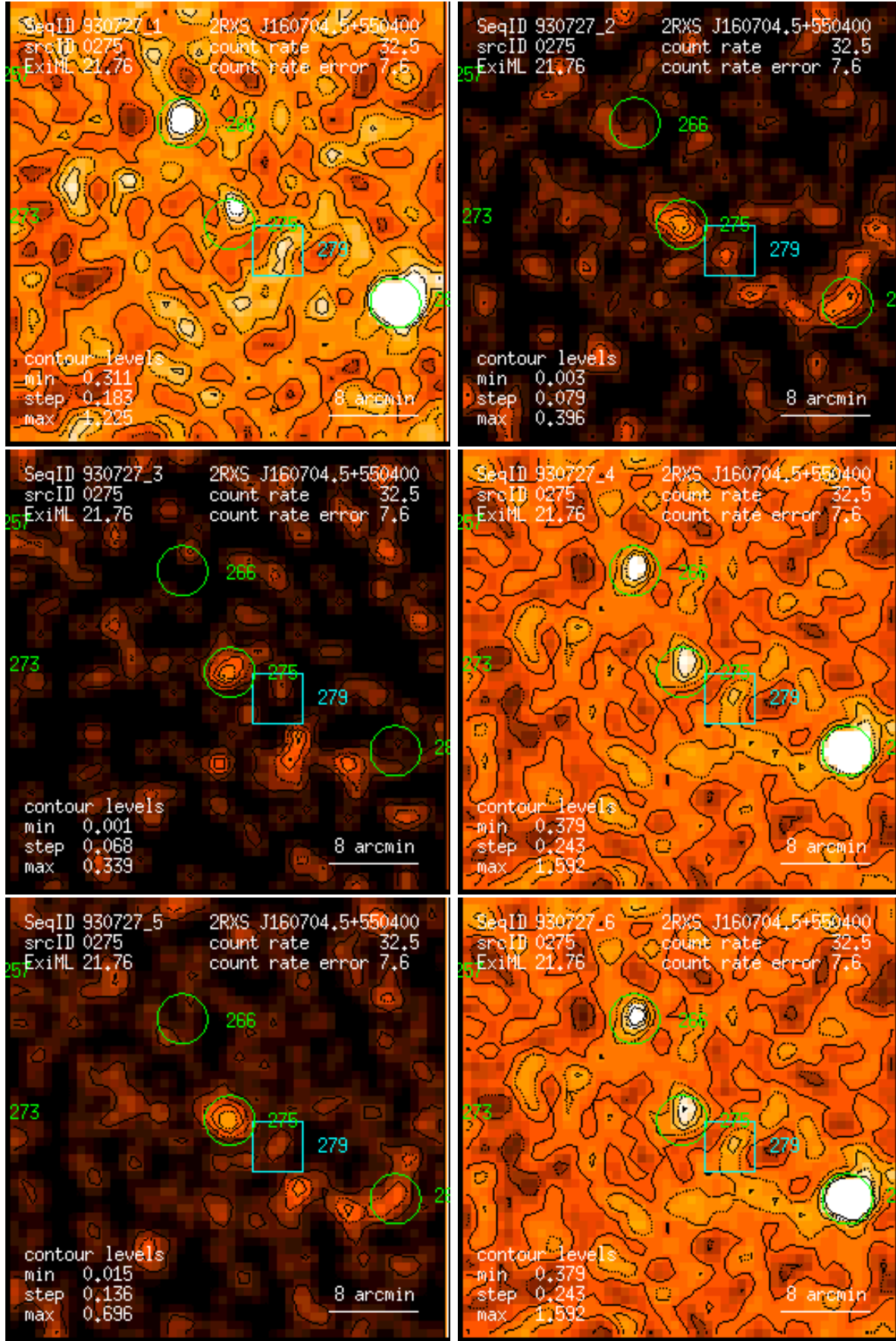
Figure 275: RASS 930727: detection 0275: band rate images, Gaussian filter: (1) PSPC channels 11 – 41, (2) 52 – 90, (3) 91 – 201, (4) 11 – 235, (5) 52 – 201, (6) 11 – 201. Broad band rates in counts/ks. Band rate contour levels in counts/ks/arcmin 2 .
