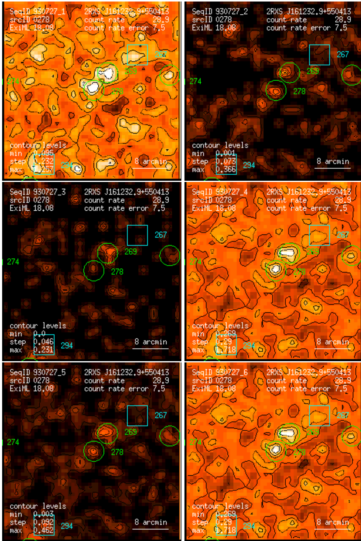
Figure 278: RASS 930727: detection 0278: band rate images, Gaussian filter: (1) PSPC channels 11 – 41, (2) 52 – 90, (3) 91 – 201, (4) 11 – 235, (5) 52 – 201, (6) 11 – 201. Broad band rates in counts/ks. Band rate contour levels in counts/ks/arcmin 2 .
