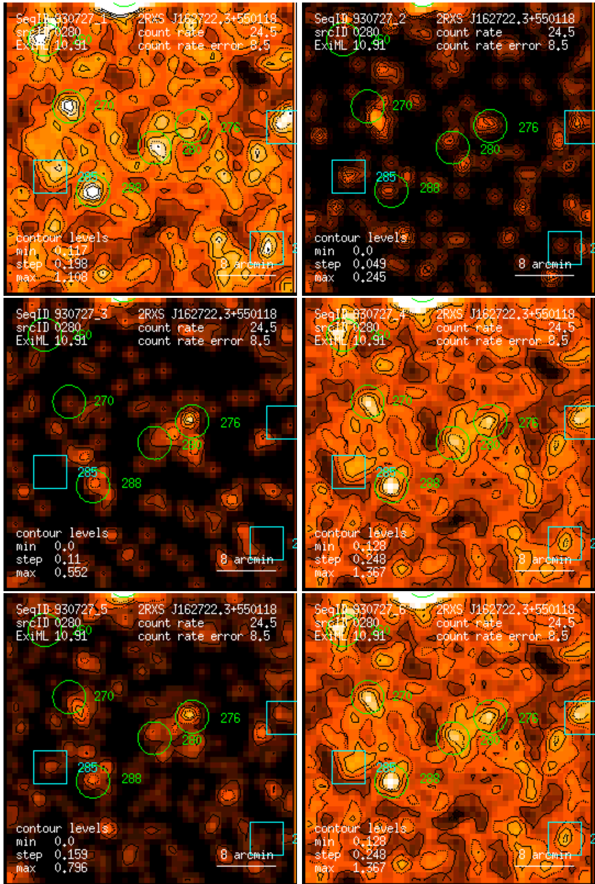
Figure 280: RASS 930727: detection 0280: band rate images, Gaussian filter: (1) PSPC channels 11 – 41, (2) 52 – 90, (3) 91 – 201, (4) 11 – 235, (5) 52 – 201, (6) 11 – 201. Broad band rates in counts/ks. Band rate contour levels in counts/ks/arcmin 2 .
