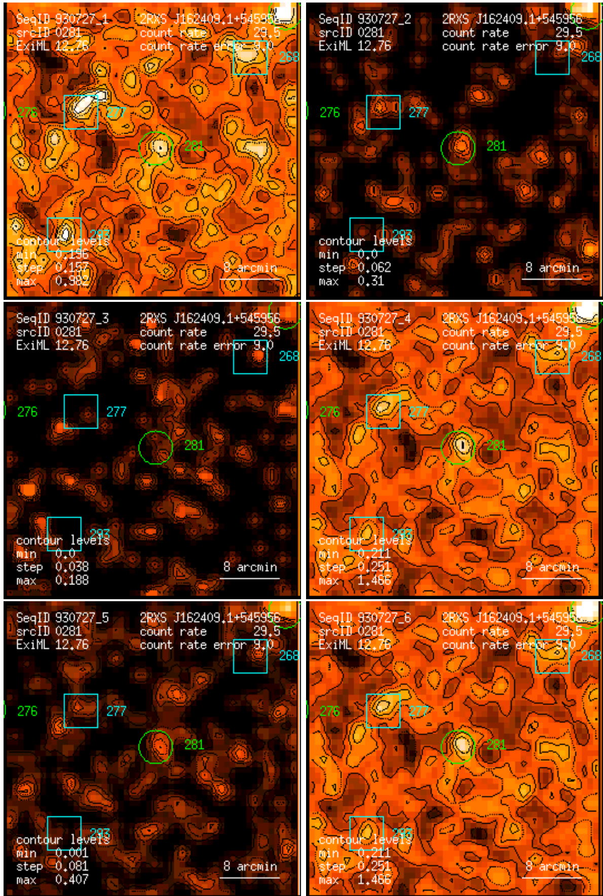
Figure 281: RASS 930727: detection 0281: band rate images, Gaussian filter: (1) PSPC channels 11 – 41, (2) 52 – 90, (3) 91 – 201, (4) 11 – 235, (5) 52 – 201, (6) 11 – 201. Broad band rates in counts/ks. Band rate contour levels in counts/ks/arcmin 2 .
