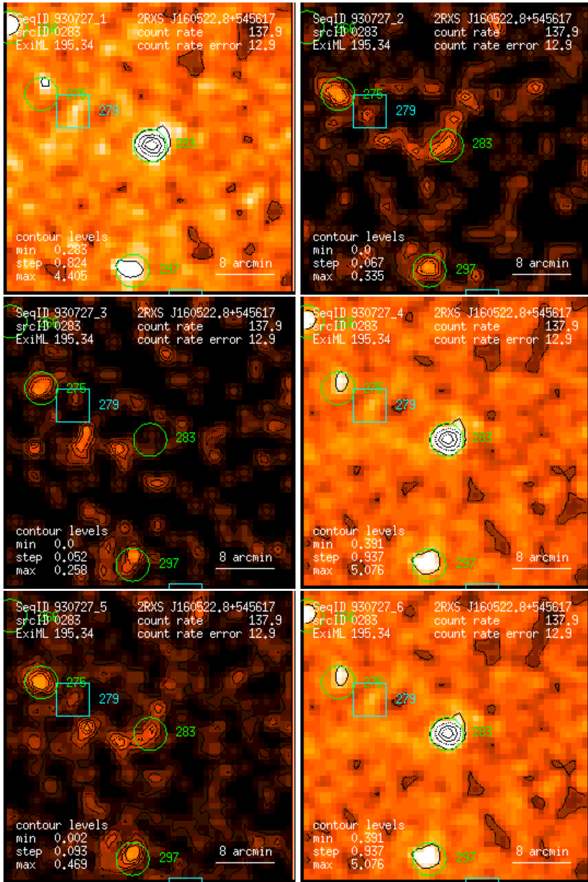
Figure 283: RASS 930727: detection 0283: band rate images, Gaussian filter: (1) PSPC channels 11 – 41, (2) 52 – 90, (3) 91 – 201, (4) 11 – 235, (5) 52 – 201, (6) 11 – 201. Broad band rates in counts/ks. Band rate contour levels in counts/ks/arcmin 2 .
