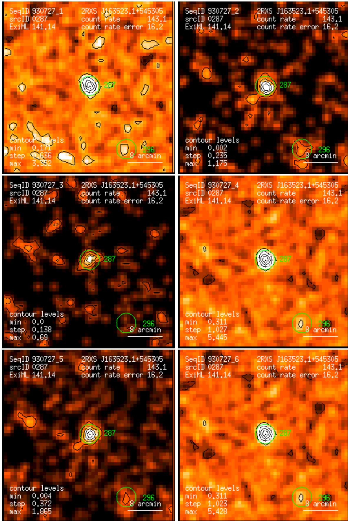
Figure 287: RASS 930727: detection 0287: band rate images, Gaussian filter: (1) PSPC channels 11 – 41, (2) 52 – 90, (3) 91 – 201, (4) 11 – 235, (5) 52 – 201, (6) 11 – 201. Broad band rates in counts/ks. Band rate contour levels in counts/ks/arcmin 2 .
