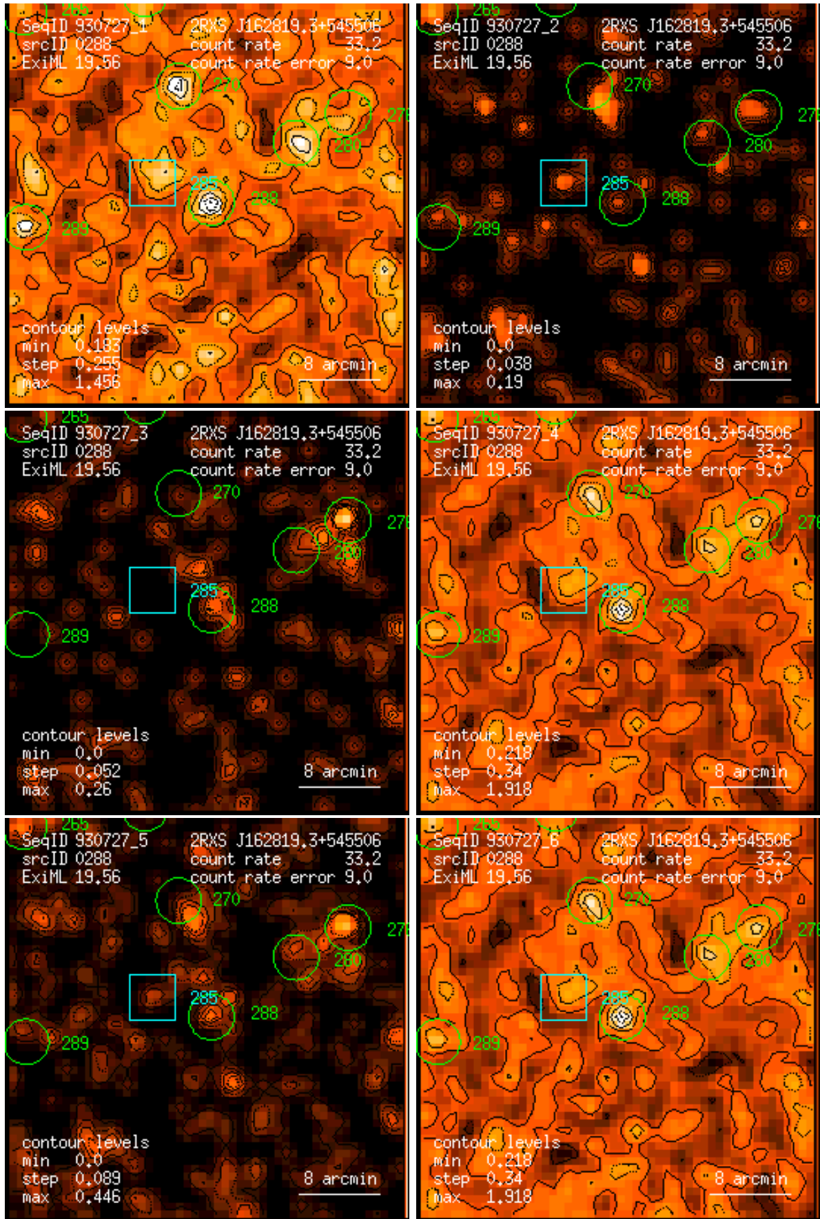
Figure 288: RASS 930727: detection 0288: band rate images, Gaussian filter: (1) PSPC channels 11 – 41, (2) 52 – 90, (3) 91 – 201, (4) 11 – 235, (5) 52 – 201, (6) 11 – 201. Broad band rates in counts/ks. Band rate contour levels in counts/ks/arcmin 2 .
