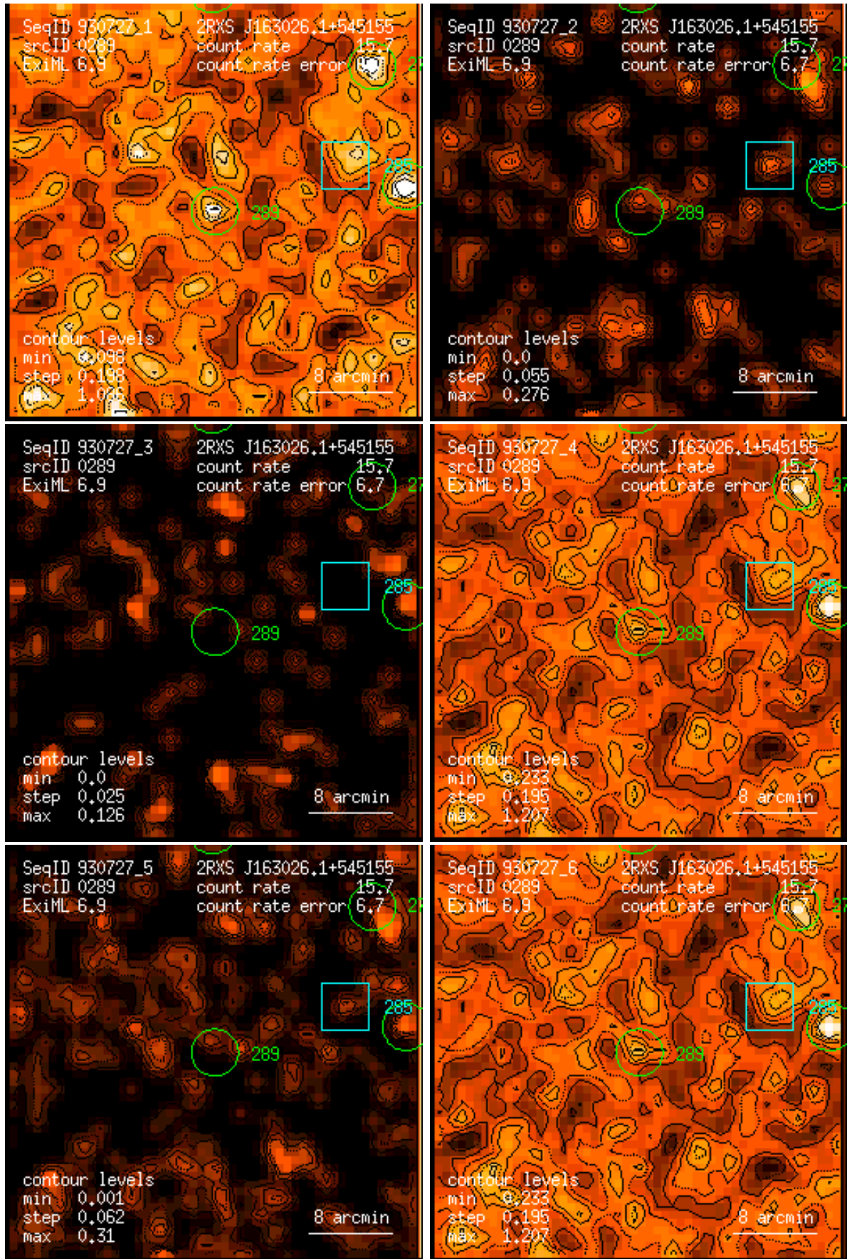
Figure 289: RASS 930727: detection 0289: band rate images, Gaussian filter: (1) PSPC channels 11 – 41, (2) 52 – 90, (3) 91 – 201, (4) 11 – 235, (5) 52 – 201, (6) 11 – 201. Broad band rates in counts/ks. Band rate contour levels in counts/ks/arcmin 2 .
