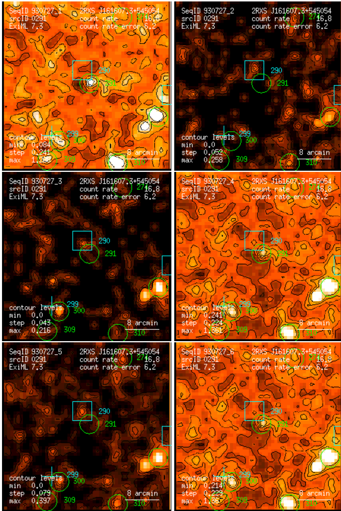
Figure 291: RASS 930727: detection 0291: band rate images, Gaussian filter: (1) PSPC channels 11 – 41, (2) 52 – 90, (3) 91 – 201, (4) 11 – 235, (5) 52 – 201, (6) 11 – 201. Broad band rates in counts/ks. Band rate contour levels in counts/ks/arcmin 2 .
