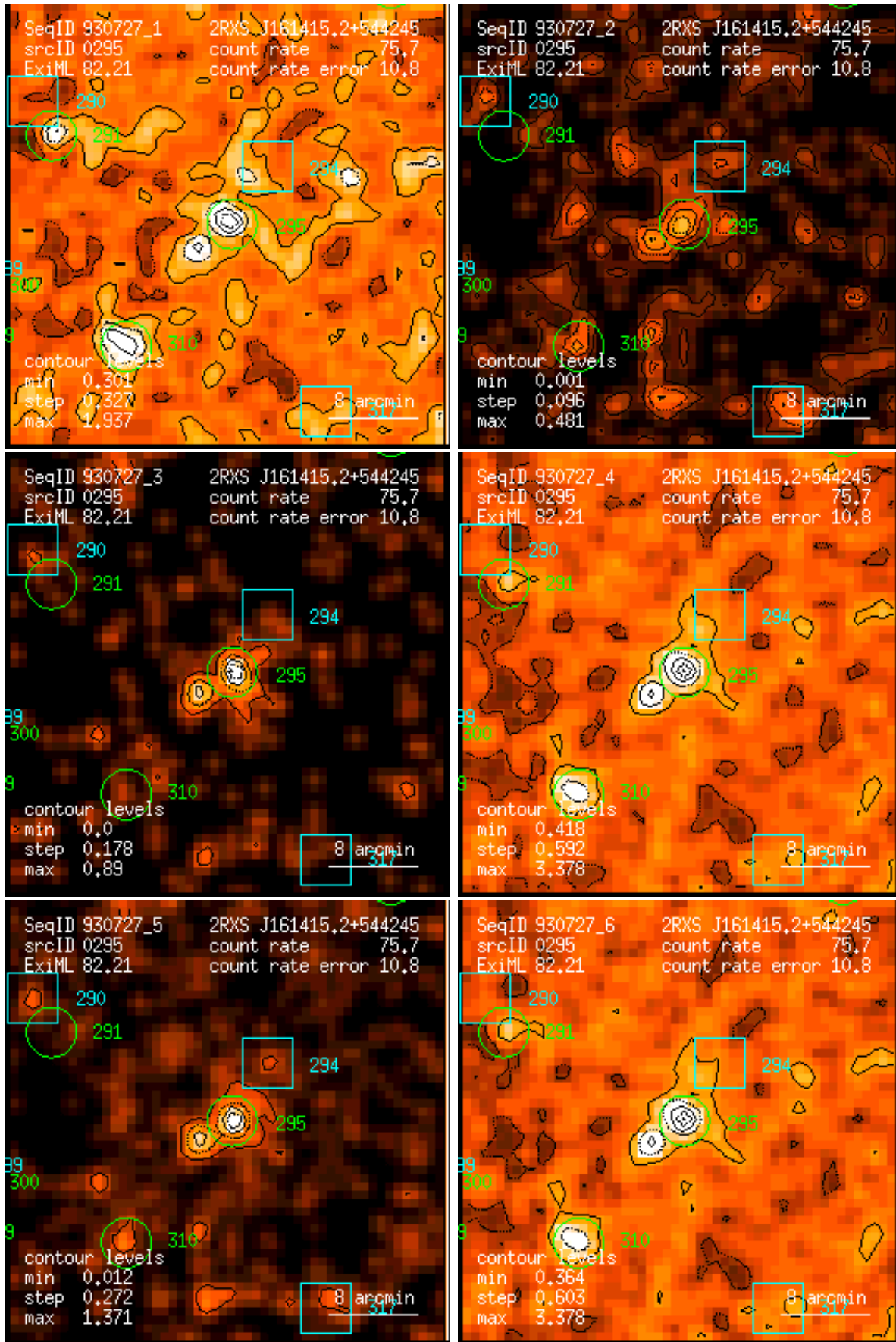
Figure 295: RASS 930727: detection 0295: band rate images, Gaussian filter: (1) PSPC channels 11 – 41, (2) 52 – 90, (3) 91 – 201, (4) 11 – 235, (5) 52 – 201, (6) 11 – 201. Broad band rates in counts/ks. Band rate contour levels in counts/ks/arcmin 2 .
