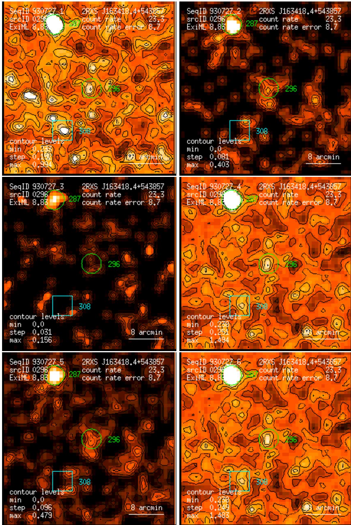
Figure 296: RASS 930727: detection 0296: band rate images, Gaussian filter: (1) PSPC channels 11 – 41, (2) 52 – 90, (3) 91 – 201, (4) 11 – 235, (5) 52 – 201, (6) 11 – 201. Broad band rates in counts/ks. Band rate contour levels in counts/ks/arcmin 2 .
