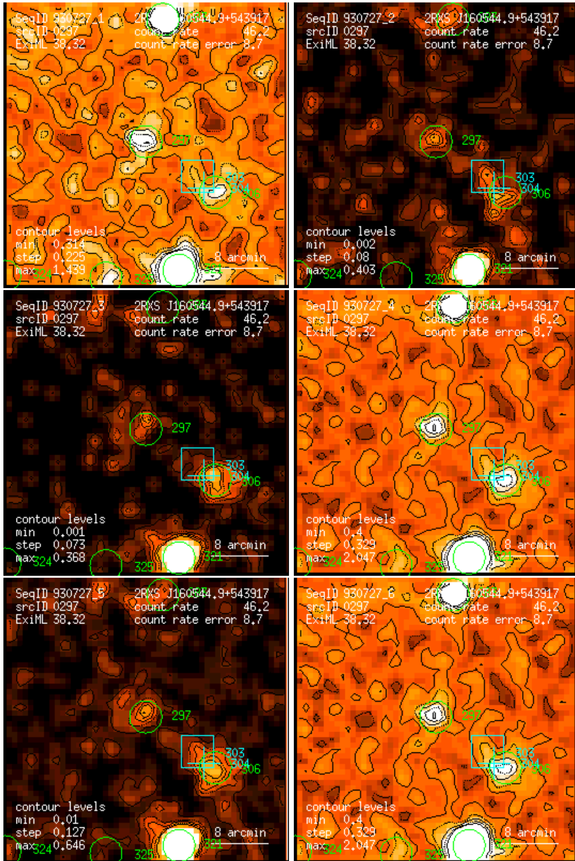
Figure 297: RASS 930727: detection 0297: band rate images, Gaussian filter: (1) PSPC channels 11 – 41, (2) 52 – 90, (3) 91 – 201, (4) 11 – 235, (5) 52 – 201, (6) 11 – 201. Broad band rates in counts/ks. Band rate contour levels in counts/ks/arcmin 2 .
