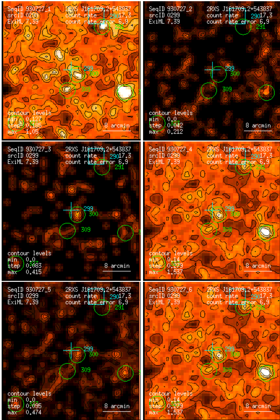
Figure 299: RASS 930727: detection 0299: band rate images, Gaussian filter: (1) PSPC channels 11 – 41, (2) 52 – 90, (3) 91 – 201, (4) 11 – 235, (5) 52 – 201, (6) 11 – 201. Broad band rates in counts/ks. Band rate contour levels in counts/ks/arcmin 2 .
