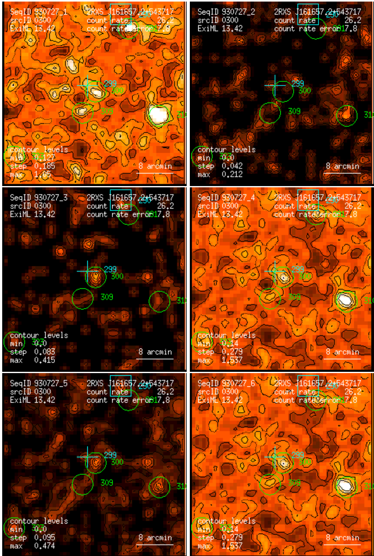
Figure 300: RASS 930727: detection 0300: band rate images, Gaussian filter: (1) PSPC channels 11 – 41, (2) 52 – 90, (3) 91 – 201, (4) 11 – 235, (5) 52 – 201, (6) 11 – 201. Broad band rates in counts/ks. Band rate contour levels in counts/ks/arcmin 2 .
