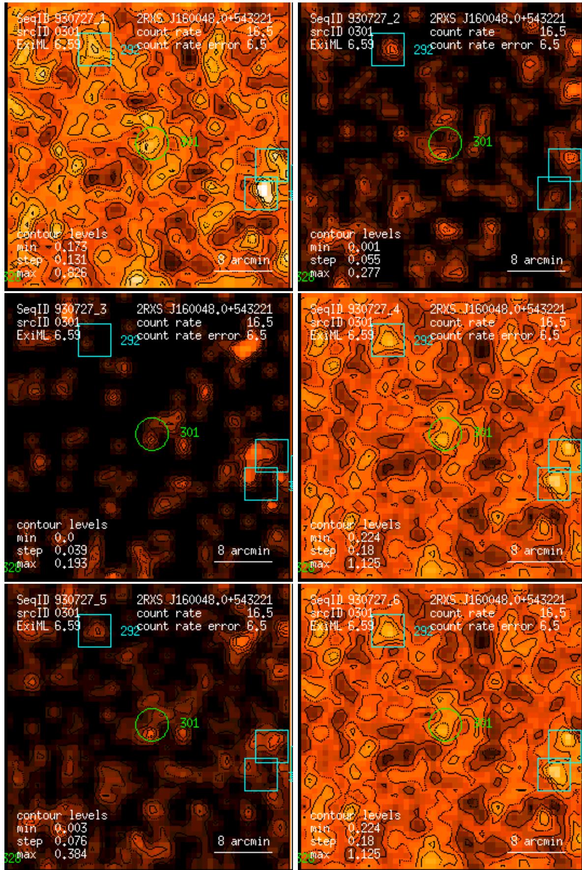
Figure 301: RASS 930727: detection 0301: band rate images, Gaussian filter: (1) PSPC channels 11 – 41, (2) 52 – 90, (3) 91 – 201, (4) 11 – 235, (5) 52 – 201, (6) 11 – 201. Broad band rates in counts/ks. Band rate contour levels in counts/ks/arcmin 2 .
